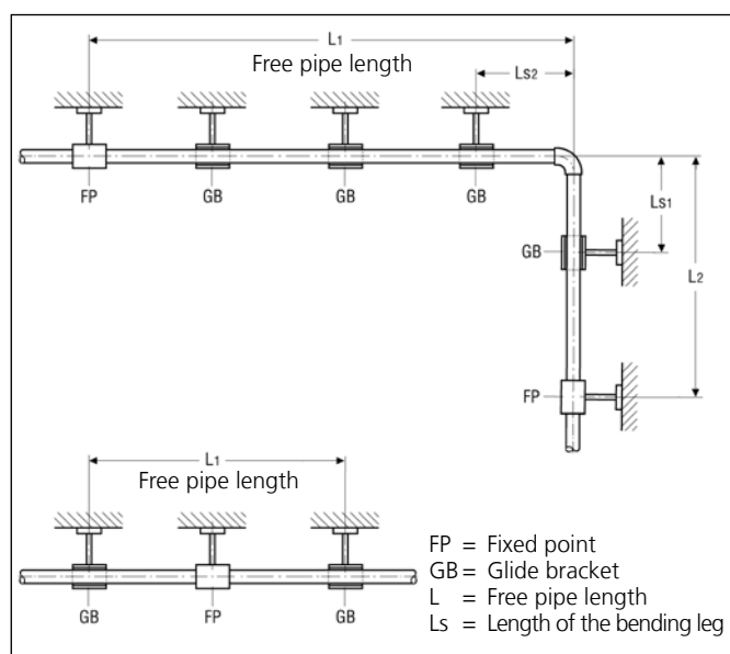
Illustration 6.1 Longitudinal expansion
