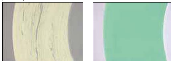
Illustration 3.4 Stereomicroscopic observation of pipe cross sections with poor dispersion and excellent dispersion of pigment and additives
