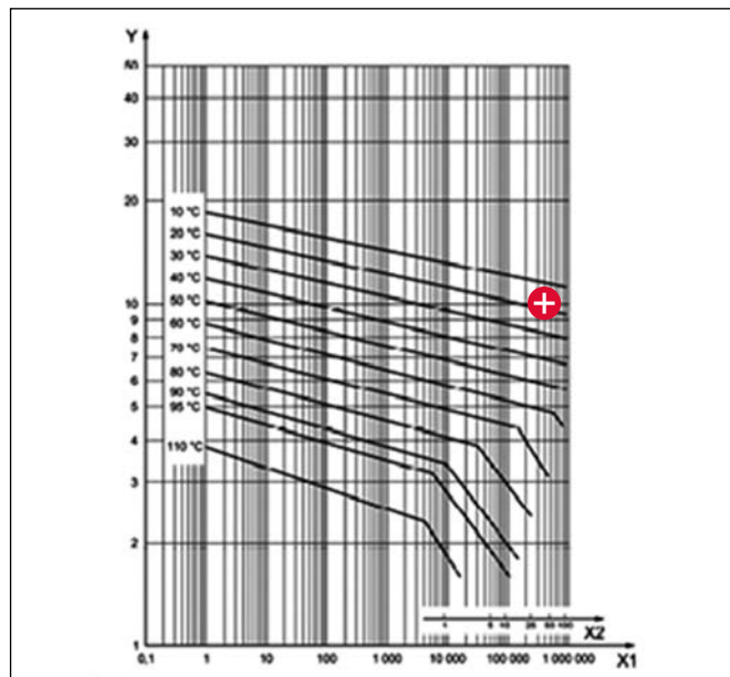
Graphic 3.1 PP-R MRS 10 MPa (20°C, 50 years)
