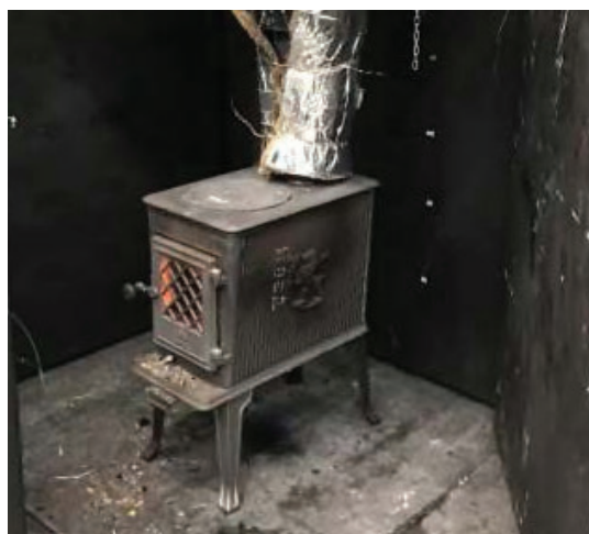
The stove on the test rig, safety test
