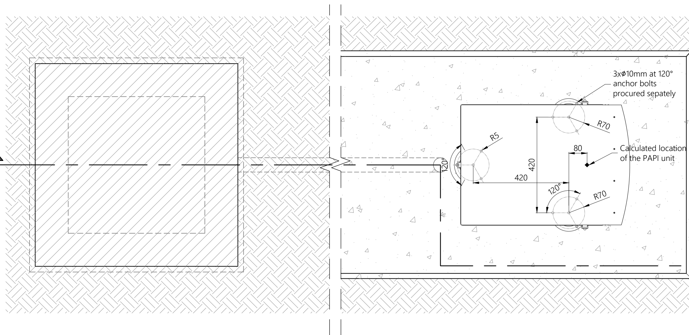
TOP VIEW PAPI Scale 1/10
