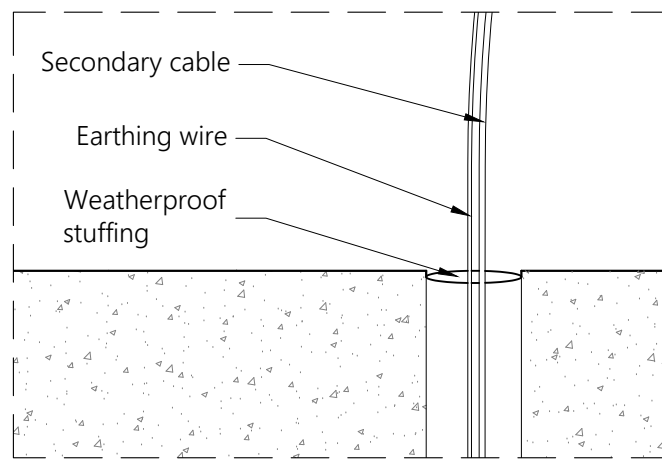
DETAIL A CLOSING OF DUCT Scale 1/5
