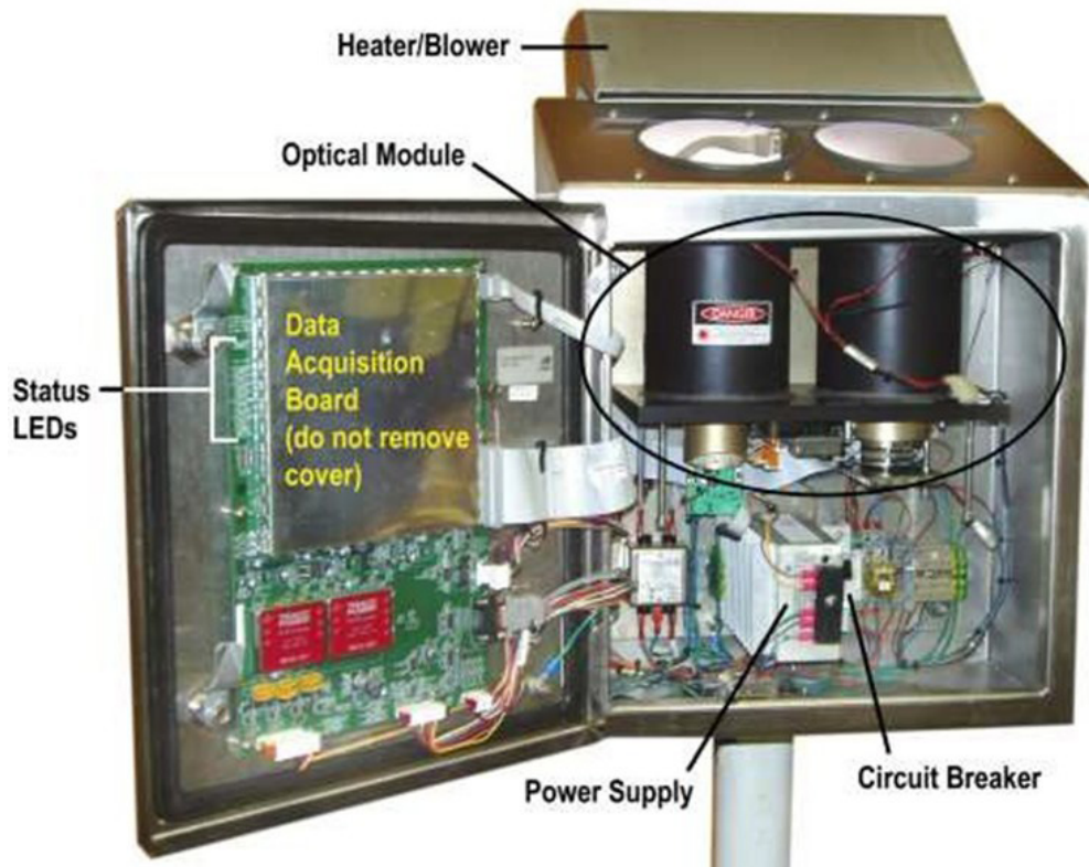
Figure 1. Ceilometer Components
