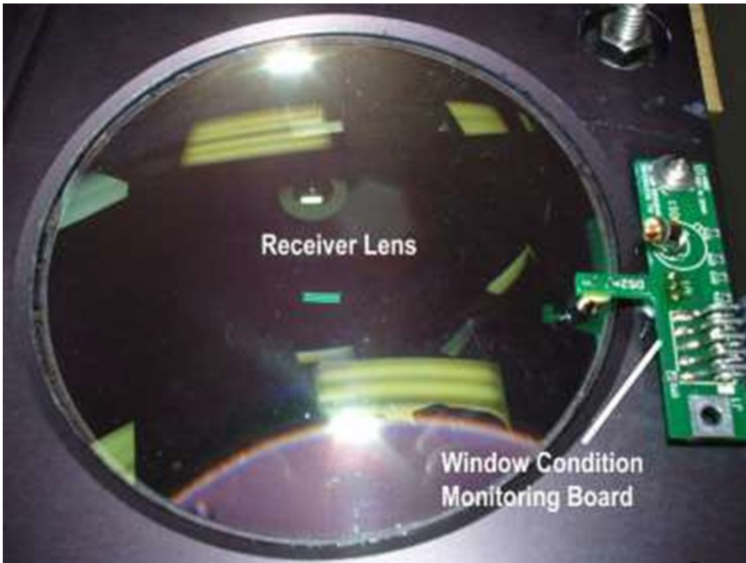
Figure 3. Window Condition Monitoring Board
