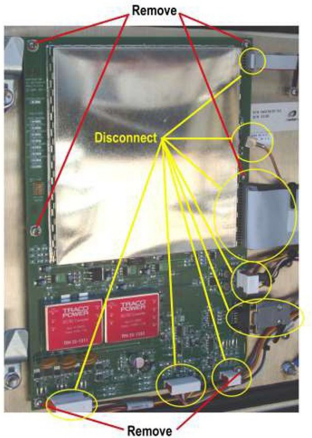
Figure 15. Data Acquisition Board Removal
