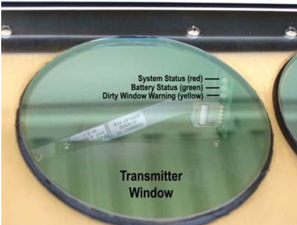
Figure 4. Ceilometer Status LEDs Location
