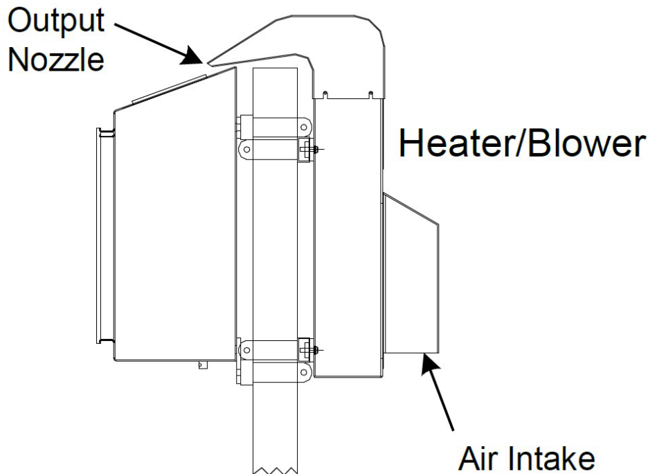
Figure 11. Heater/Blower Maintenance Areas
