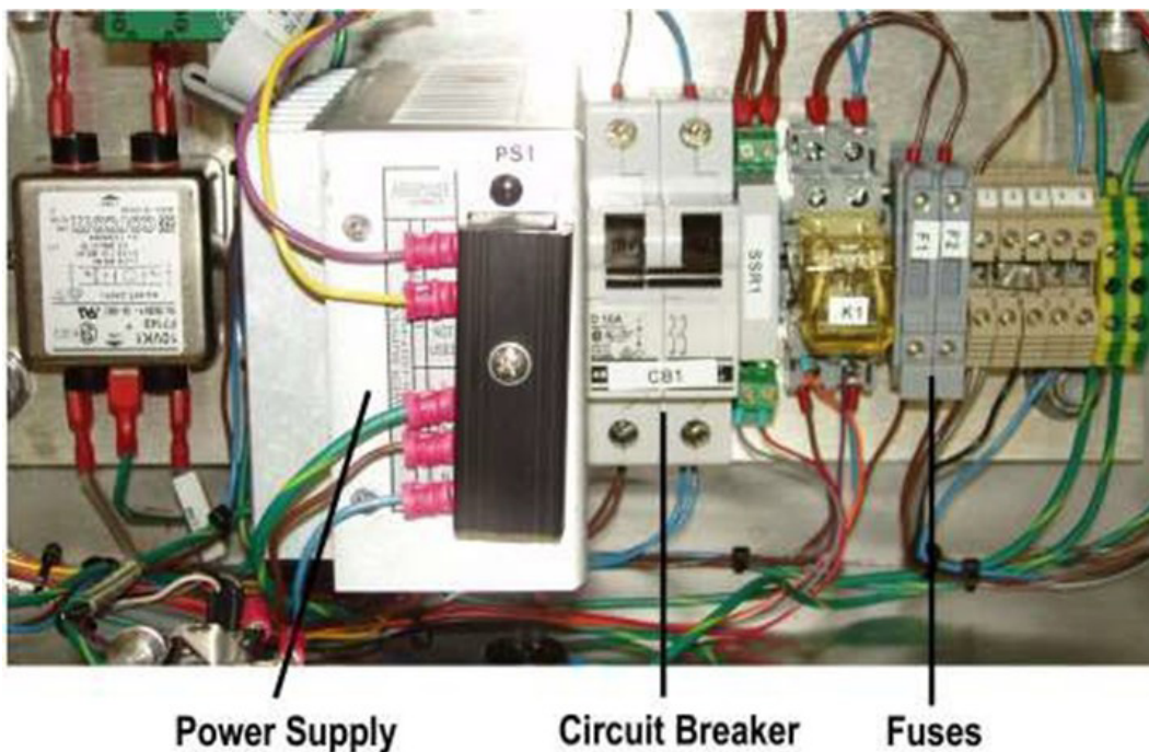
Figure 13. DIN Rail Components
