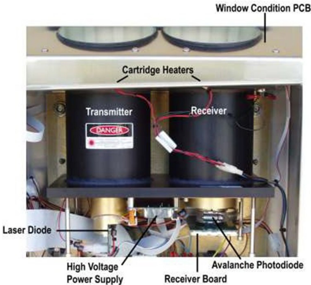
Figure 2. Optical Module
