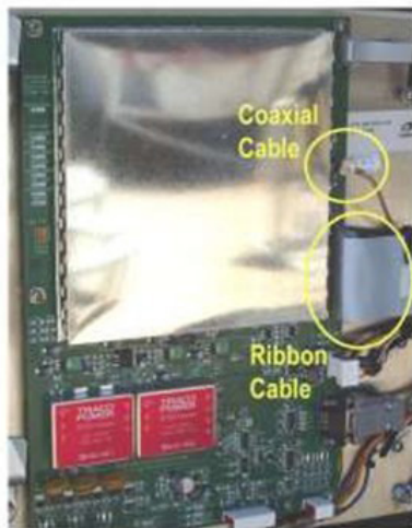
Figure 16. Optical Module Removal
