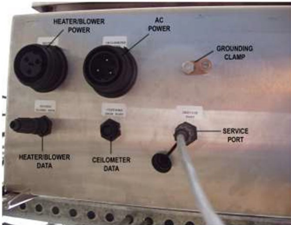
Figure 8. Ceilometer Connectors
