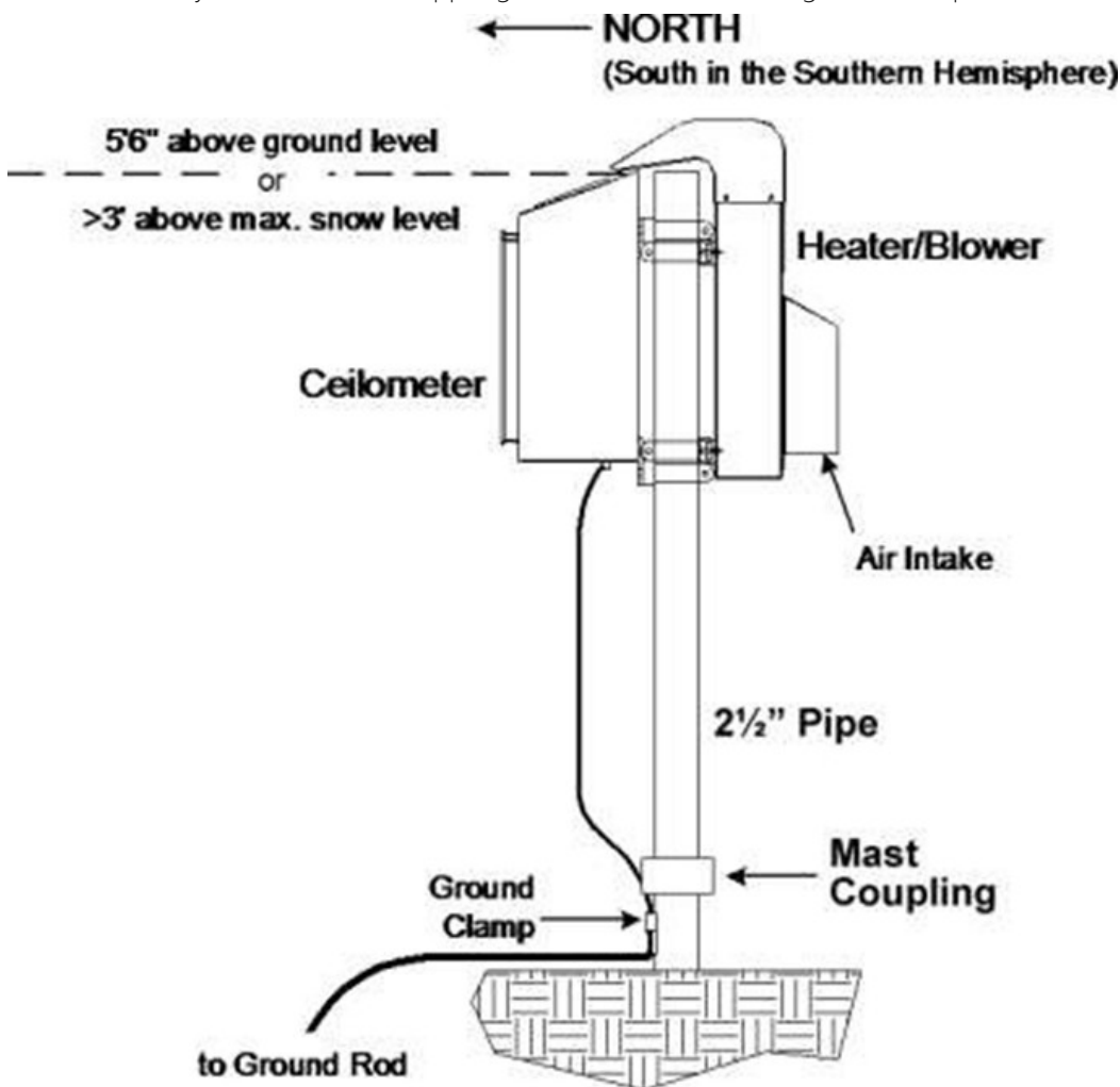
Figure 7. Ceilometer Mounting
