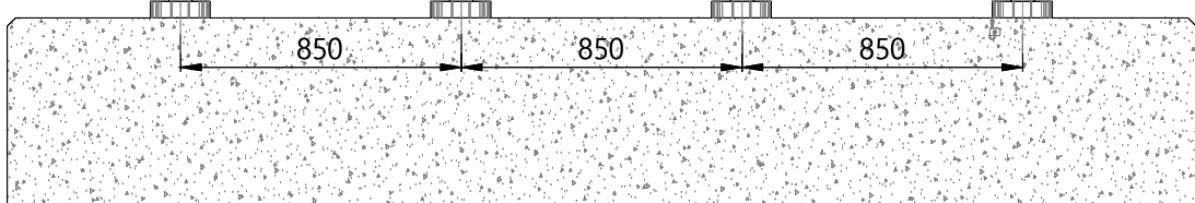
FRONT VIEW SIGN 3000x700mm Scale 1/25
