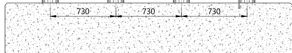
FRONT VIEW SIGN 2650x700mm Scale 1/25
