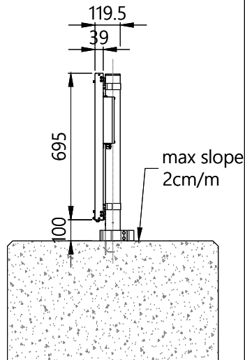
SIDE VIEW SIGN 700mm Scale 1/25
