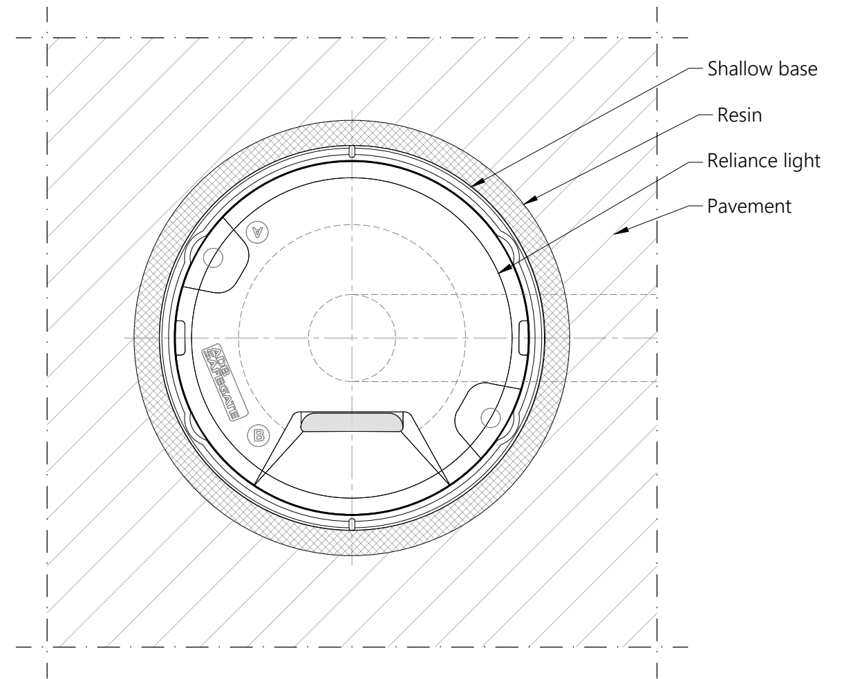
TOP VIEW RELIANCE INSET 8" UNIDIRECTIONAL LIGHT Scale 1/3
