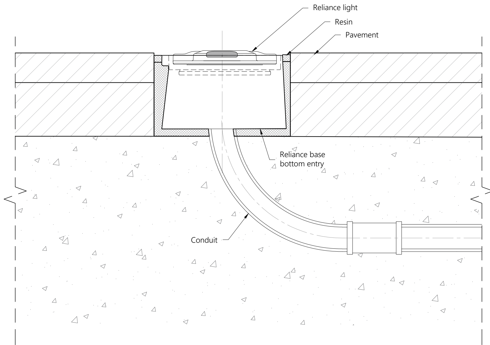
SECTION RELIANCE INSET 8" UNIDIRECTIONAL LIGHT Scale 1/4
