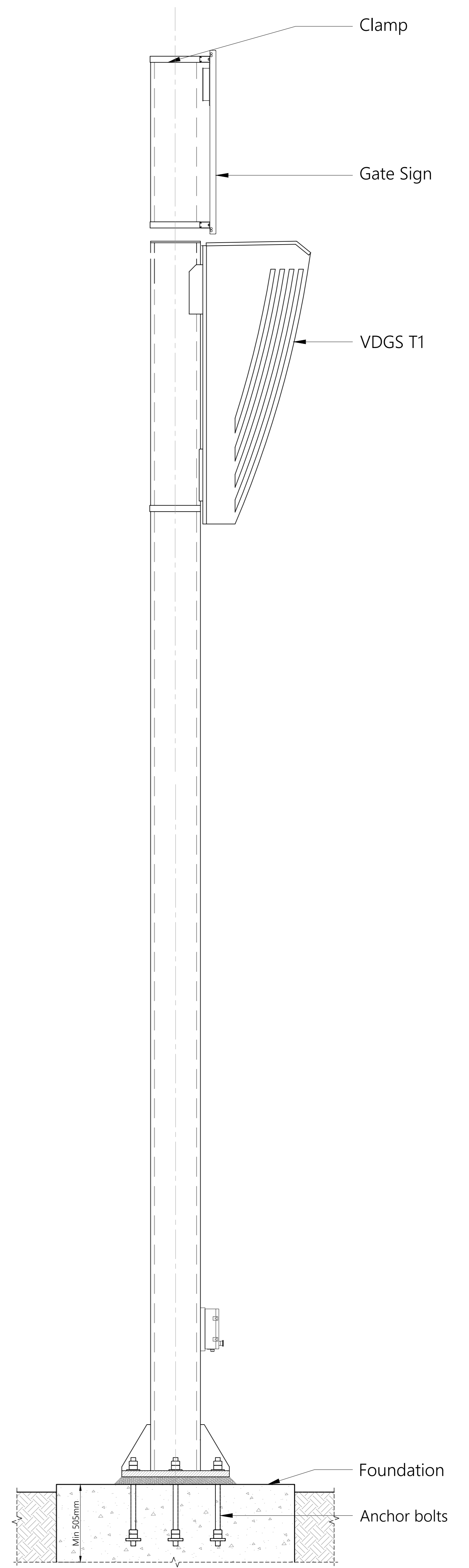
SIDE VIEW A-VDGS T1
