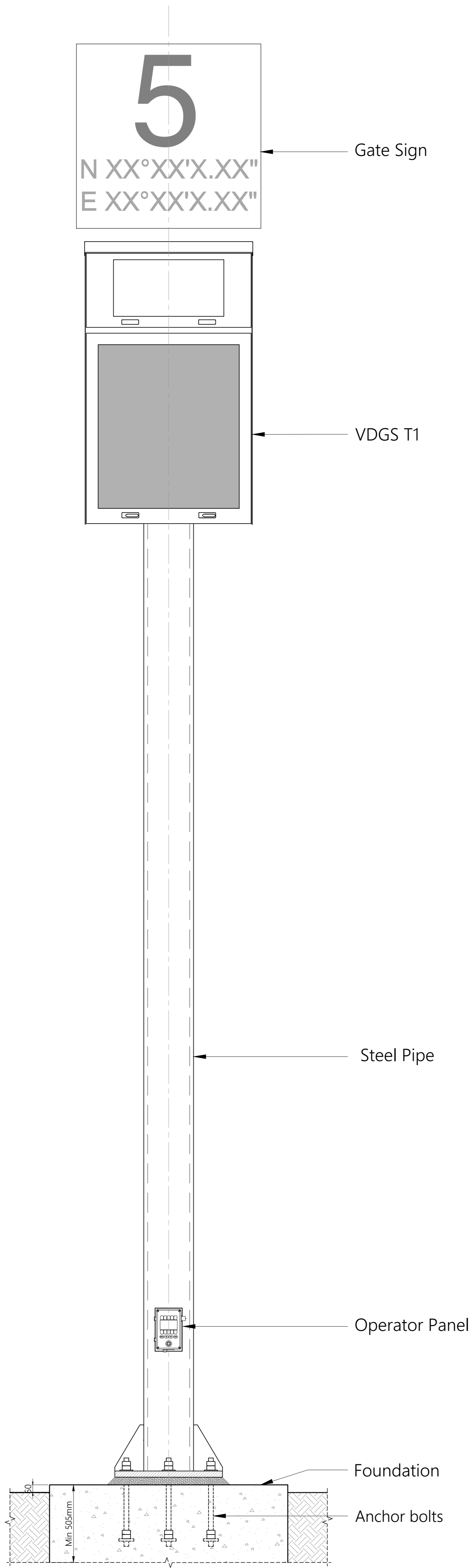
FRONT VIEW A-VDGS T1
