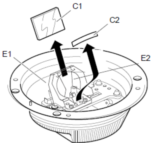
Figure 11: Filter replacement procedure
