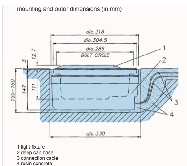
Figure 3: Installation drawing
