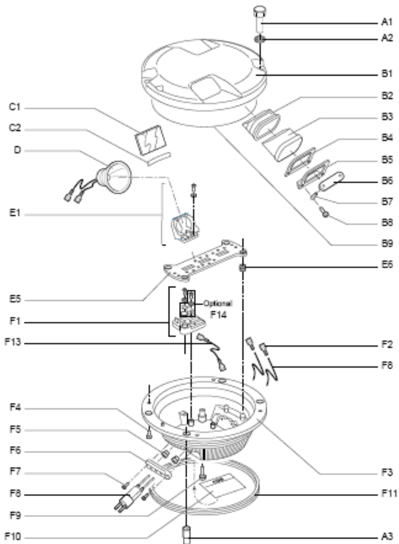
Figure 18: 8-inch F-Range inset light - Exploded View 1
