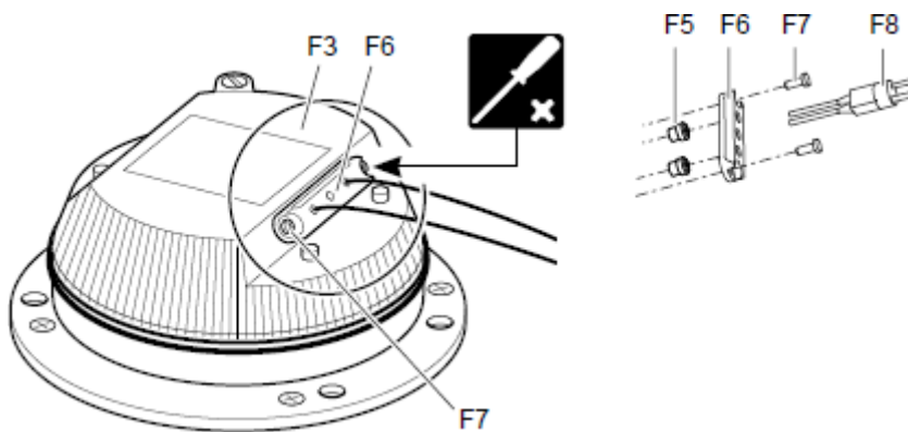
Figure 15: Cable assembly replacement procedure
