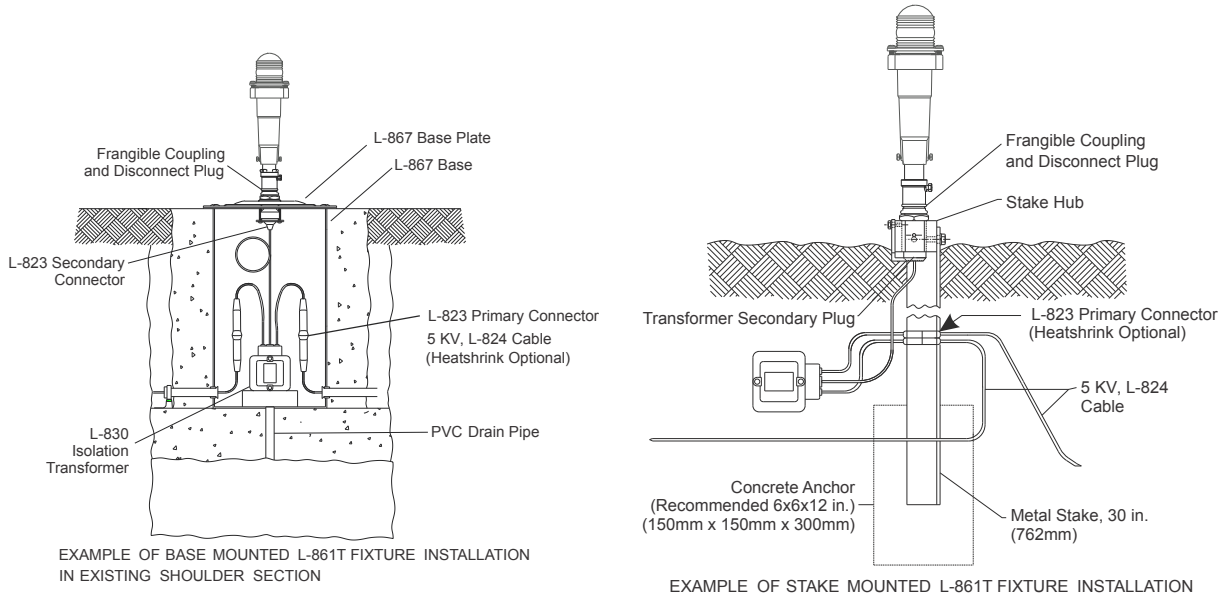
Figure 1: Installation Example
