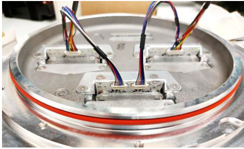
Figure 42: Three prisms (unidirectional)
