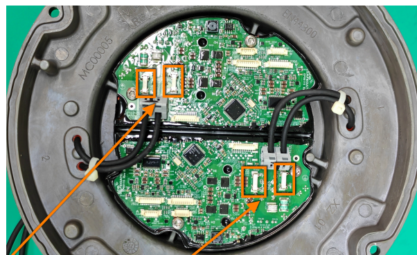
Figure 10: 2-connector converter (4 fuse resistors)
