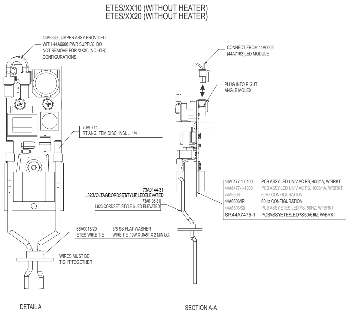
Figure 8: L-861T ETES Fixture and L-861T ETES (without heater)
