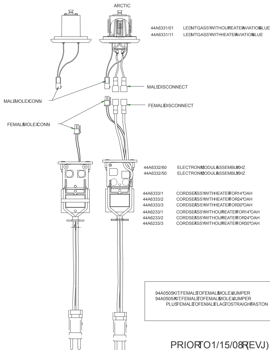
Figure 12: ETES LED Retro Fit Chart Prior to 1/15/08 Rev J
