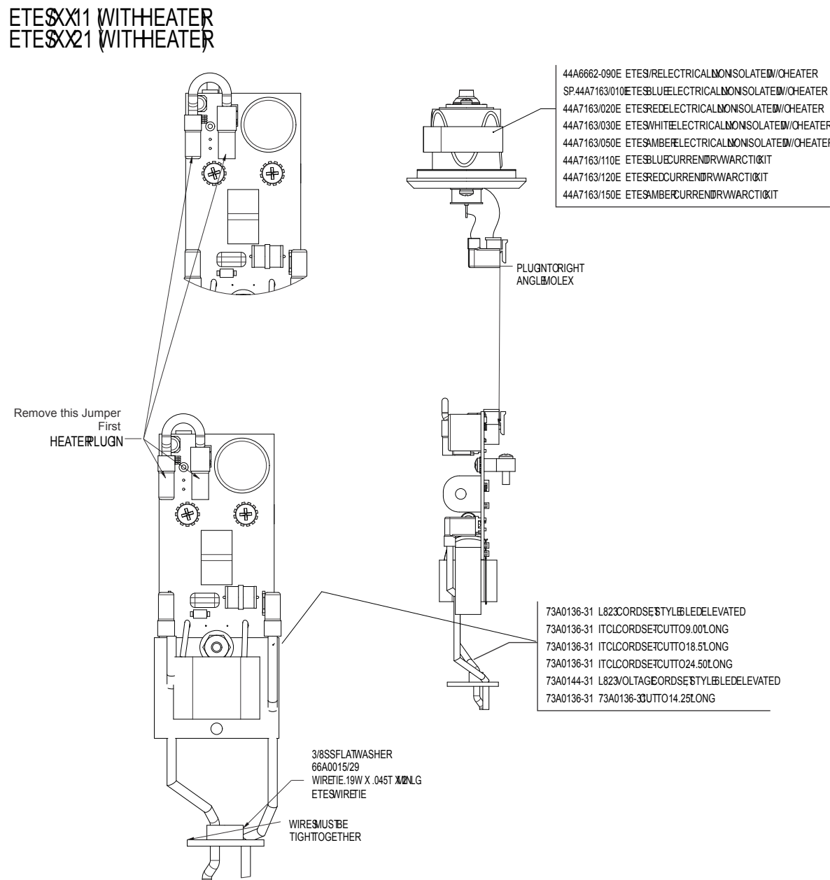
Figure 9: L-861T ETES (with heater)
