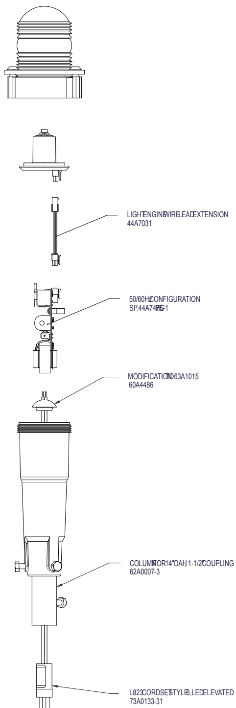
Figure 5: RELIANCE ETES Assembly
