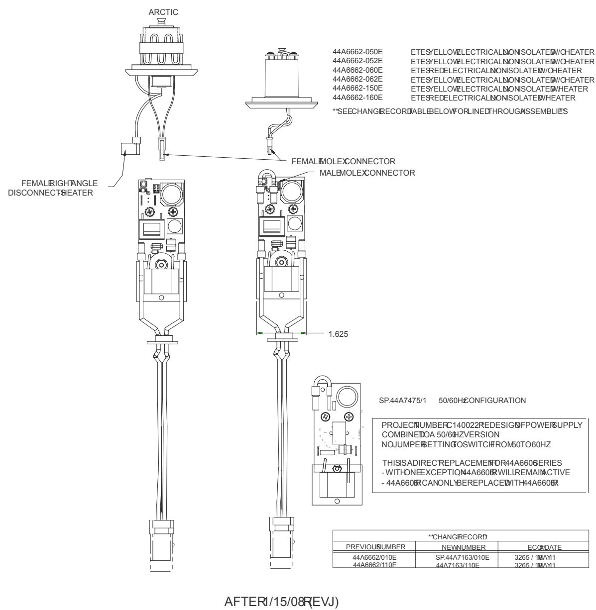
Figure 11: ETES LED Retro Fit Chart to Rev J and After 1/15/08
