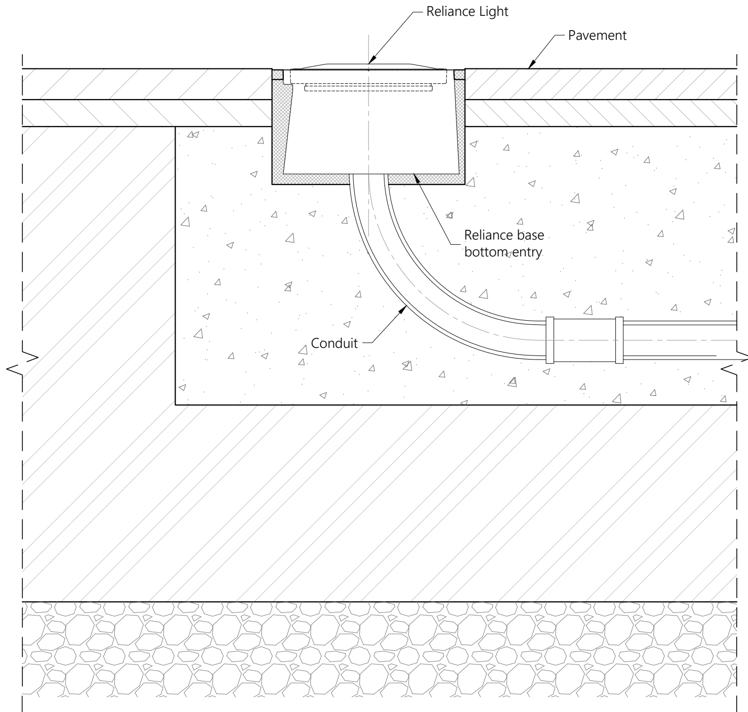
SECTION RELIANCE INSET 8" OMNIDIRECTIONAL LIGHT (4 windows) Scale 1/5
