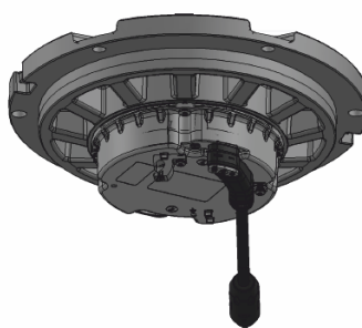
Taxiway Inset 12" with Style-1 jacketed cord set
