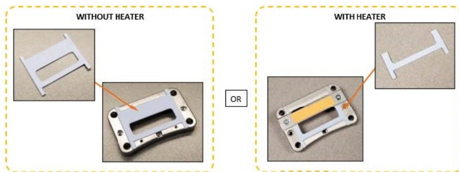
Figure 49: Light engine without and with heater
