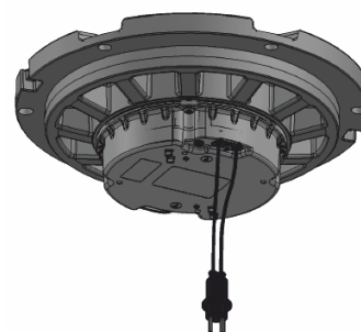
Taxiway Inset 12" with Style-6 cord set
