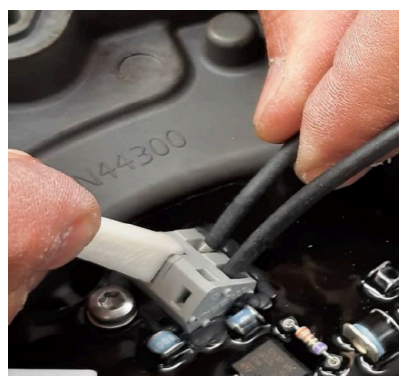
Figure 34: Releasing/locking secondary wires with insert tool
