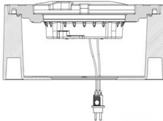
Figure 2: In a 12-in base with adapter ring
