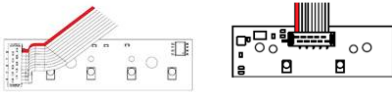
Figure 15: LED board
