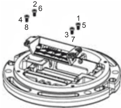
Figure 20: Tighten screws in sequence
