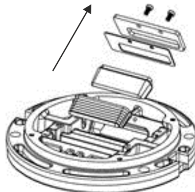
Figure 17: Remove prism and gasket
