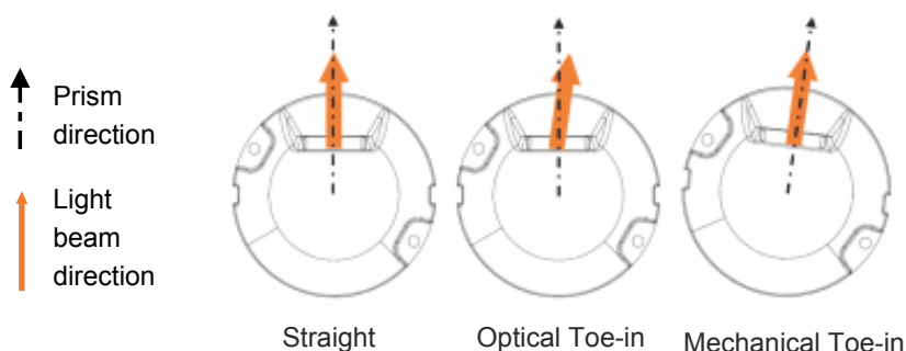
Figure 3: Toe-in
