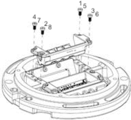
Figure 14: Tighten screws
