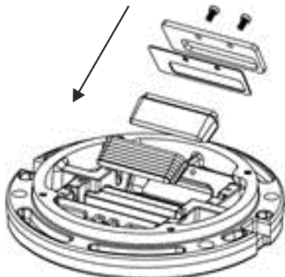
Figure 18: New prism into prism gasket
