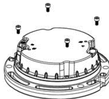
Figure 12: Tighten screws
