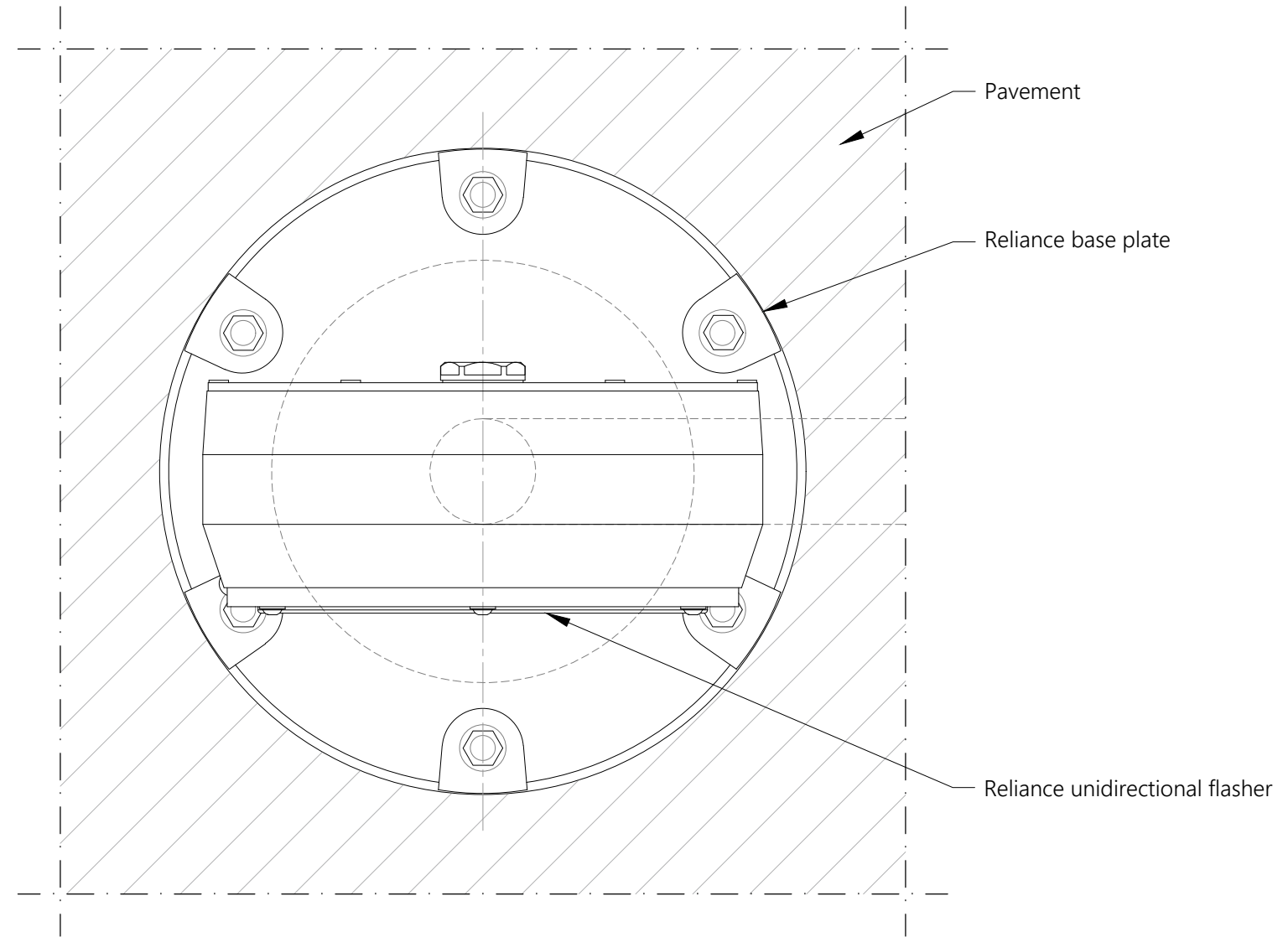
○ TOP VIEW RELIANCE ELEVATED UNIDIRECTIONAL FLASHER Scale 1/3
