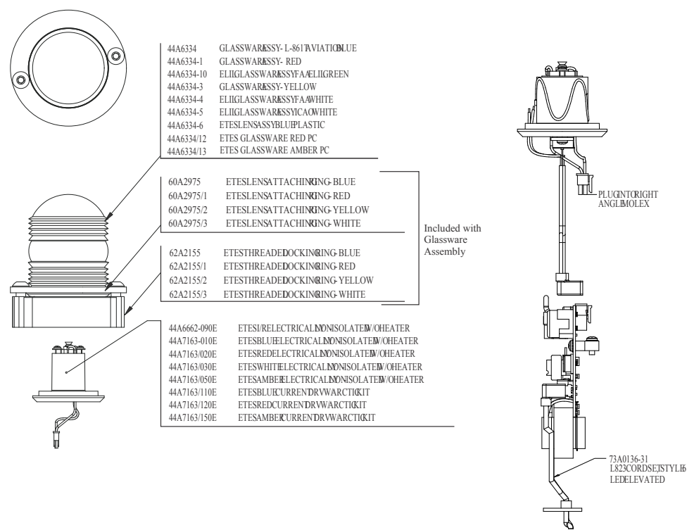
Figure 6: L-861T ETES Fixture (part 1 of 2)
