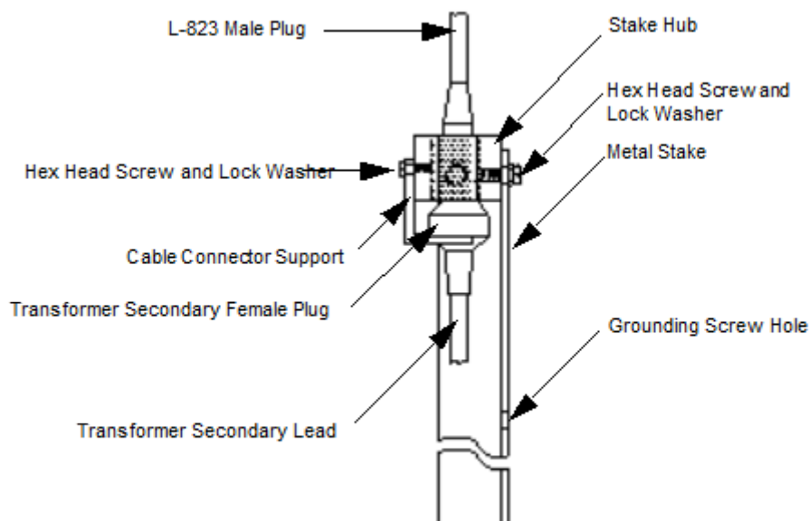
Figure 4: Stake Assembly
