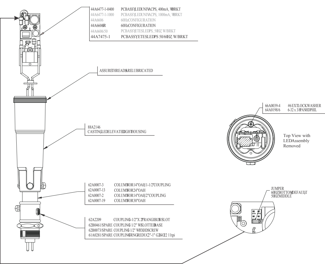
Figure 7: L-861T ETES Fixture (part 2 of 2)
