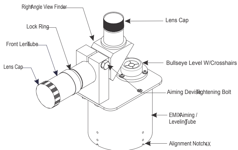
Figure 2: Alignment Tool
