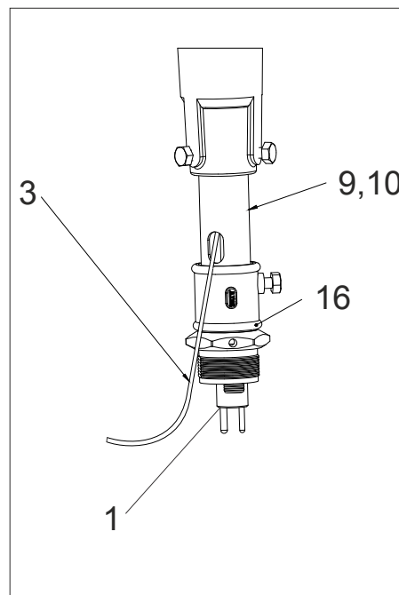
Figure 8: Earthing (Digit 5 = 6) Configurations
