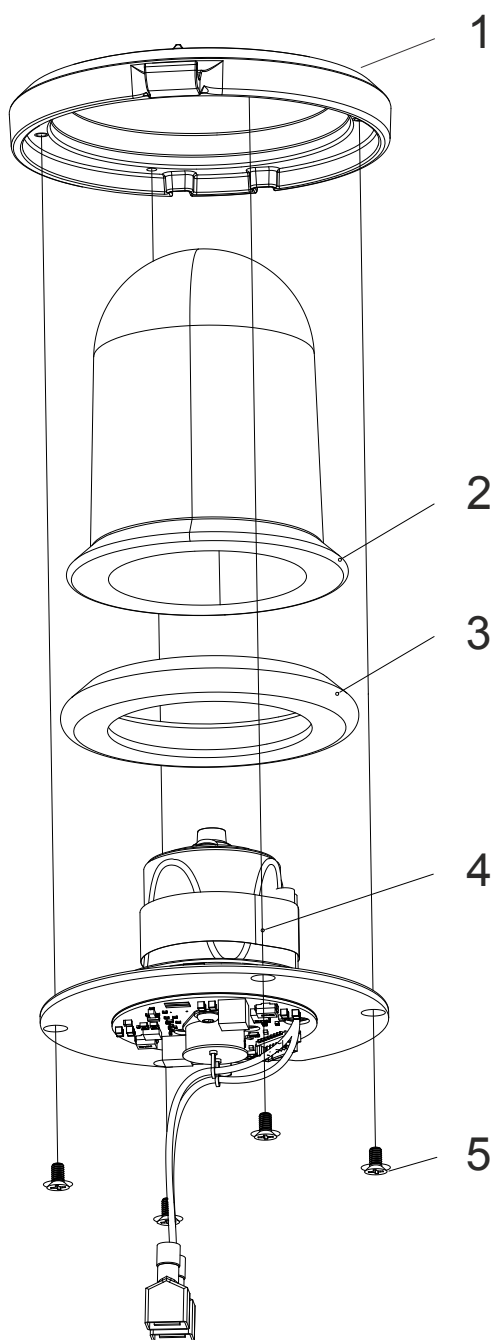
Figure 9: Optic Assembly Parts Diagram
