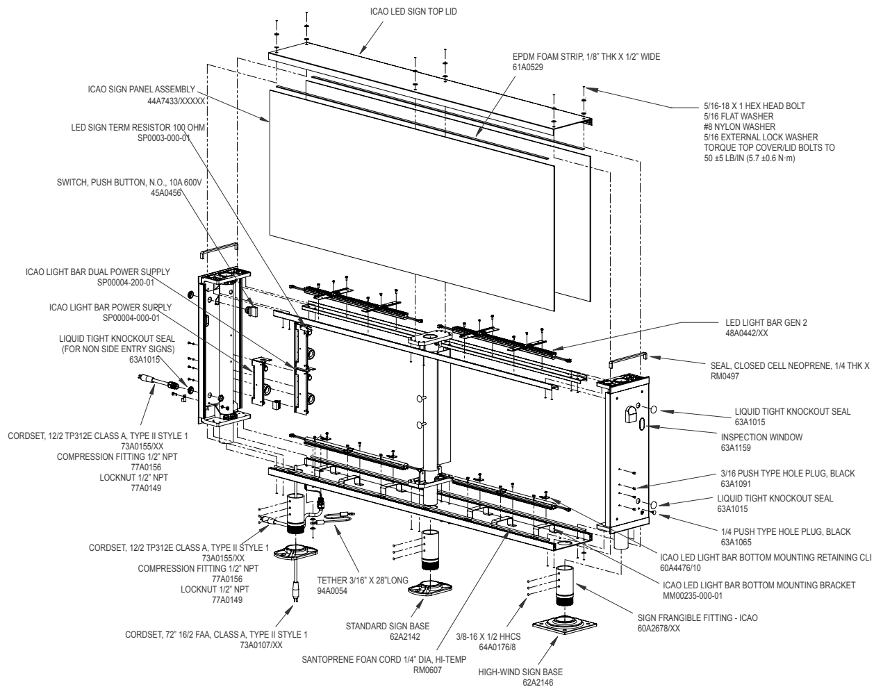
Figure 1: TP312/ICAO LED Sign Assembly Parts
