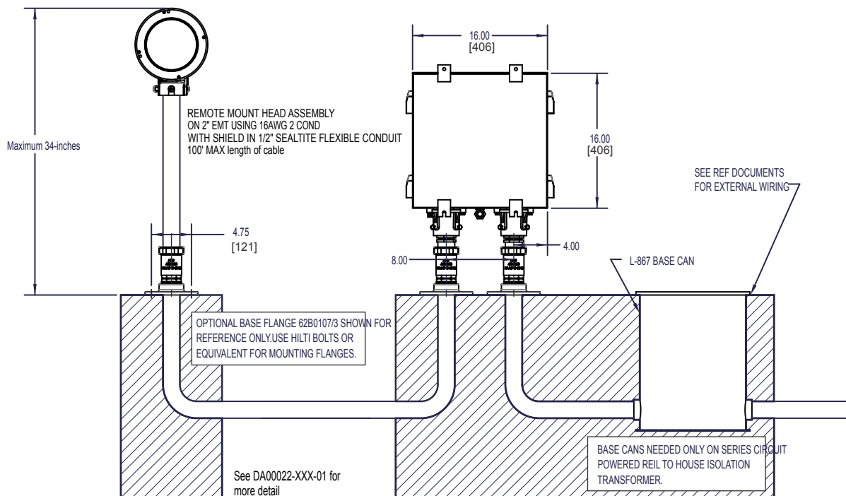
Figure 5: Remote Mounted Head Configuration
