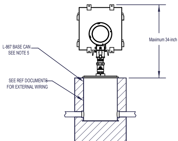
Figure 3: One-Leg Mounting Configuration (alt base can mount shown)
