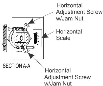
Figure 7: Horizontal Aiming (top view of flash head assembly)
