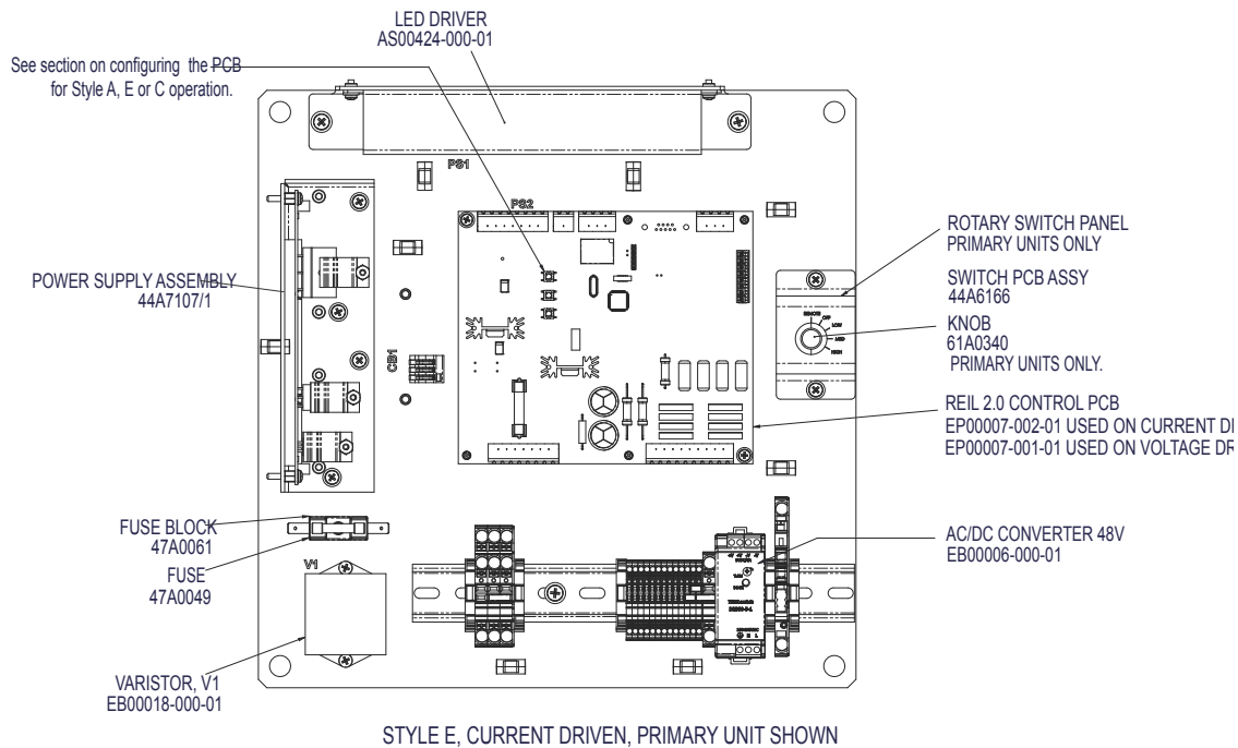
Figure 11: REIL A-E-C Current Driven Cabinet Interior
