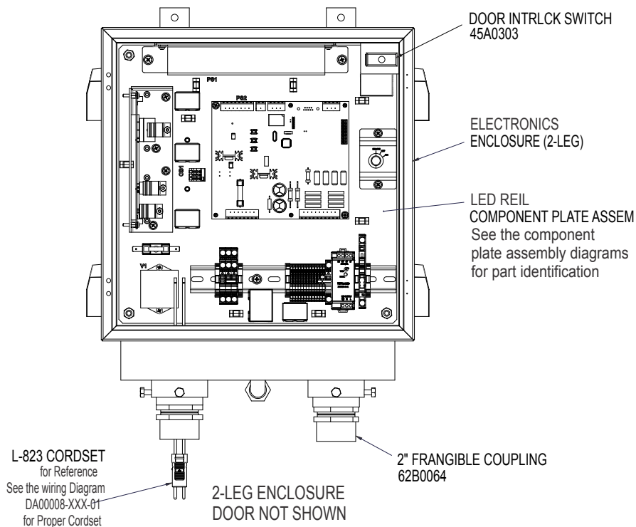
Figure 27: Enclosure Assembly Front View
