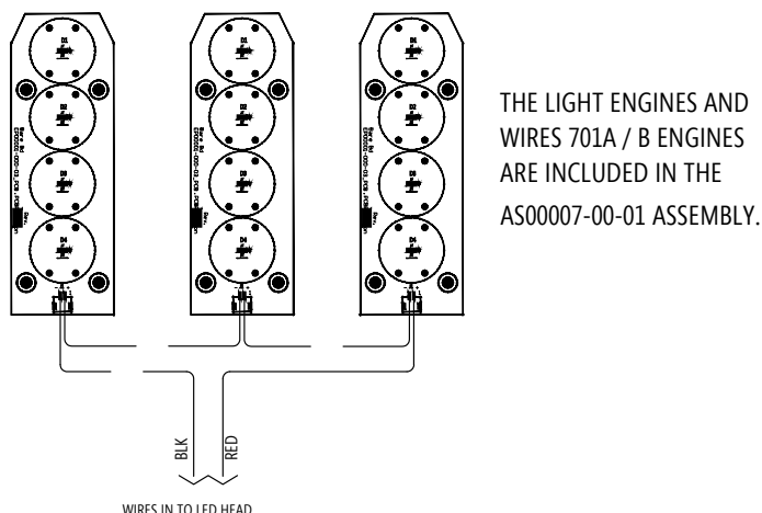
Figure 14: Primary Current-Driven LED REIL Internal Wiring Diagram (2 of 2)
