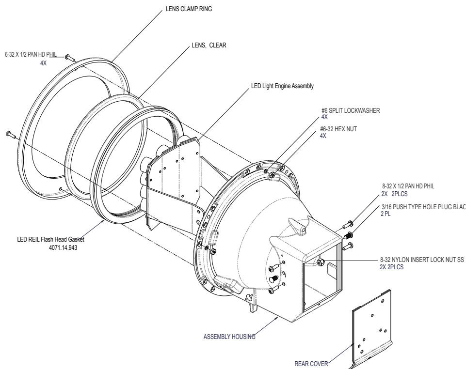
Figure 10: LED Light Engine Replacement Kit AK00014-000-01
