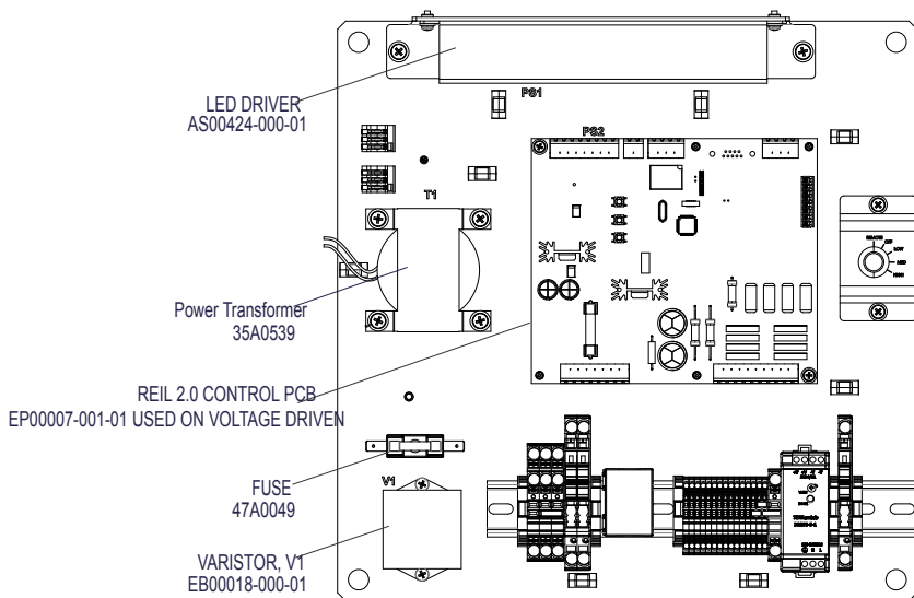
STYLE E, VOLTAGE DRIVEN, PRIMARY UNIT SHOWN
