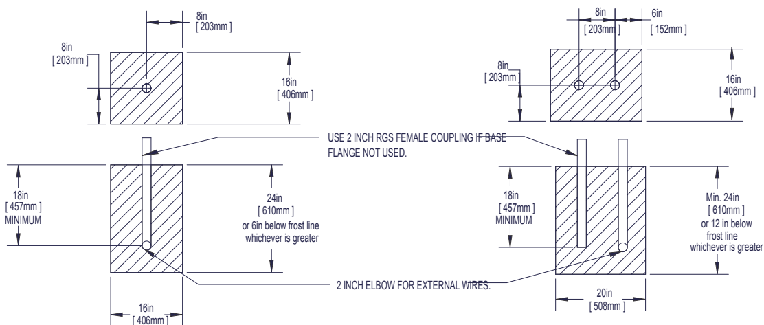
Figure 6: Cabinet Foundation Mounting Dimensions
