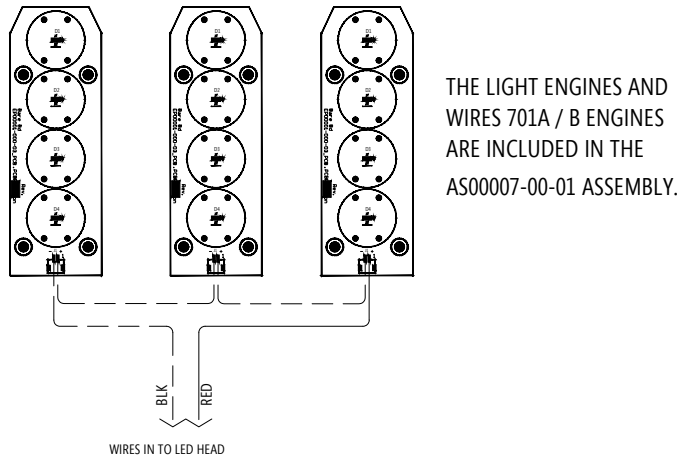
Figure 19: Primary Voltage-Driven LED REIL Internal Wiring Diagram (2 of 2)
