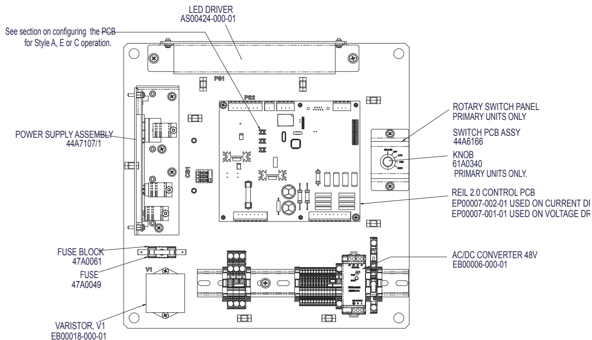
STYLE E, CURRENT DRIVEN, PRIMARY UNIT SHOWN
