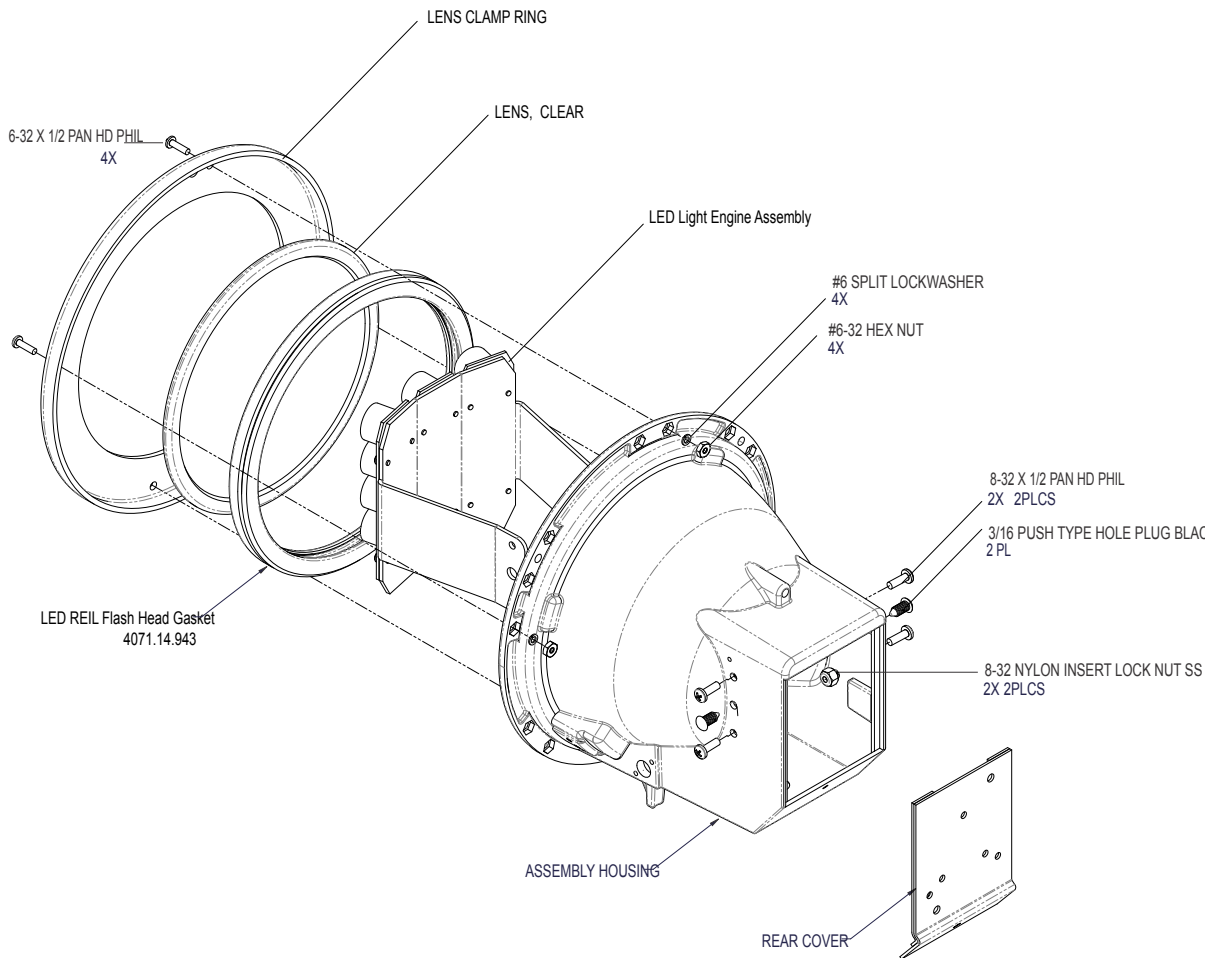
Figure 30: LED Engine Replacement Kit AK00014-000-01
