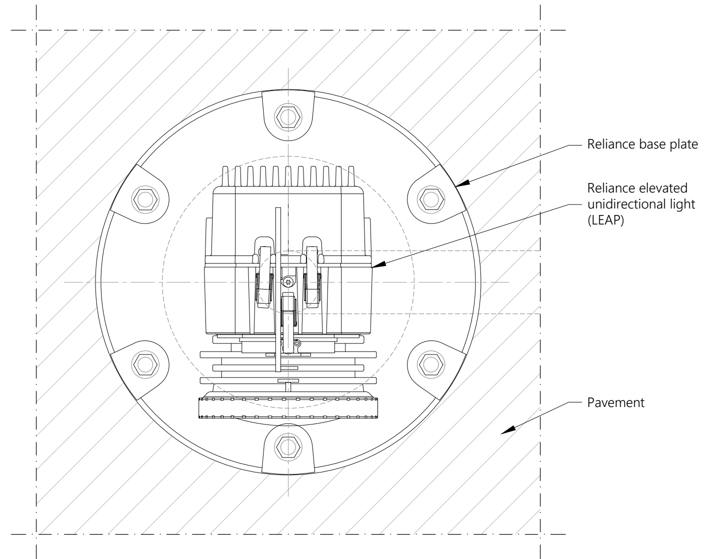
SECTION RELIANCE ELEVATED UNIDIRECTIONAL LIGHT Scale 1/3
