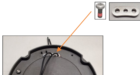
Figure 38: Dispose old bolt and cord-set-retainer disc
