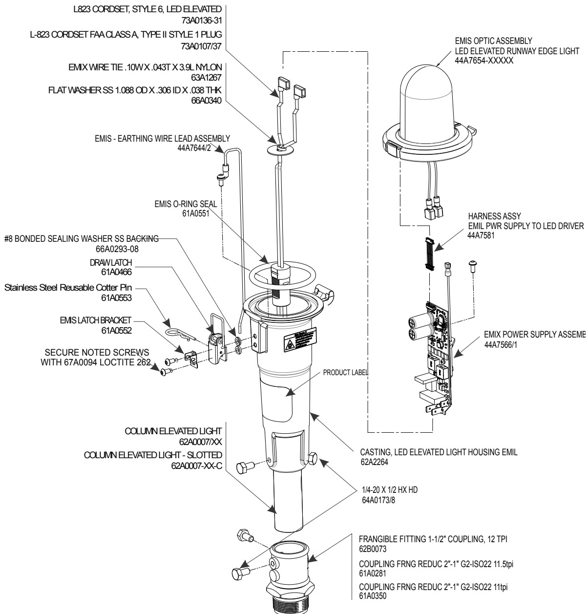
Figure 6: EMIS-L Assembly
