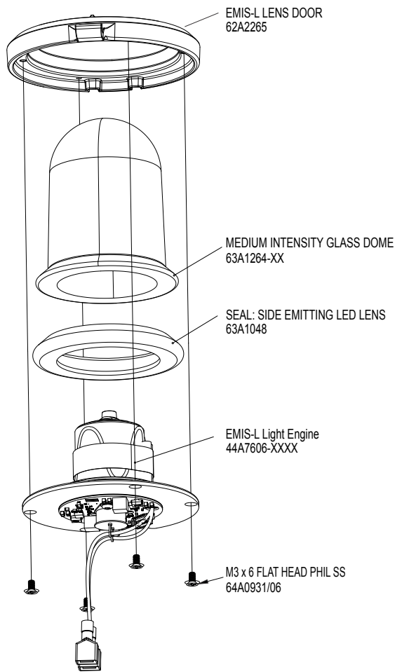
Figure 3: The EMIS-L Optic Assembly
