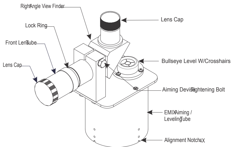
Figure 2: Alignment Tool
