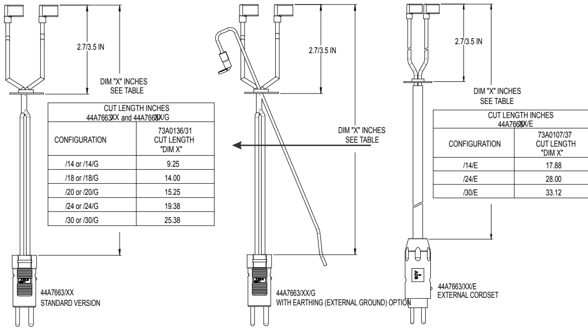
Figure 10: Cordsets
