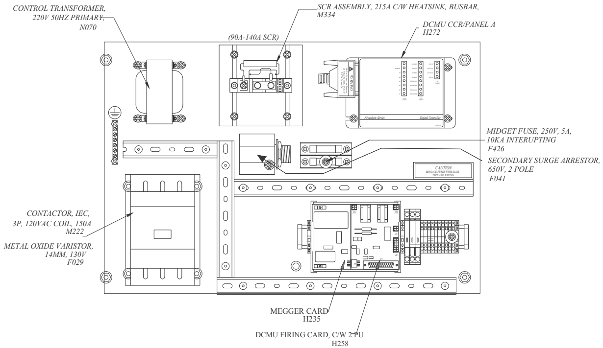
Figure 4: 20 kW Component Plate
