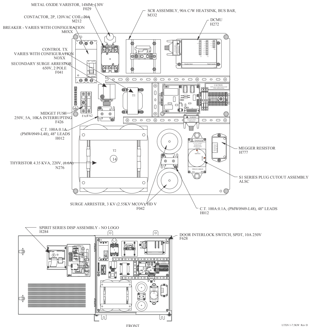
Figure 2: 1 - 7.5 Component Plate
