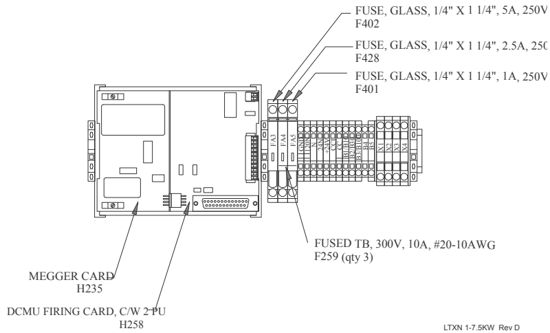
Figure 1: 1 - 30 kW terminal block parts
