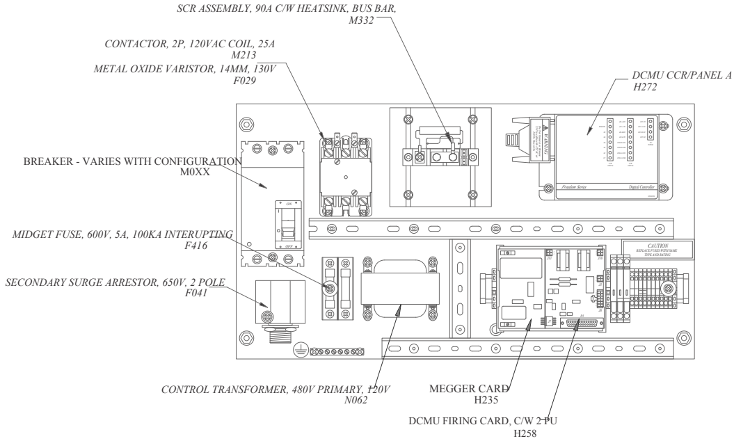
Figure 4: 20 kW Component Plate
