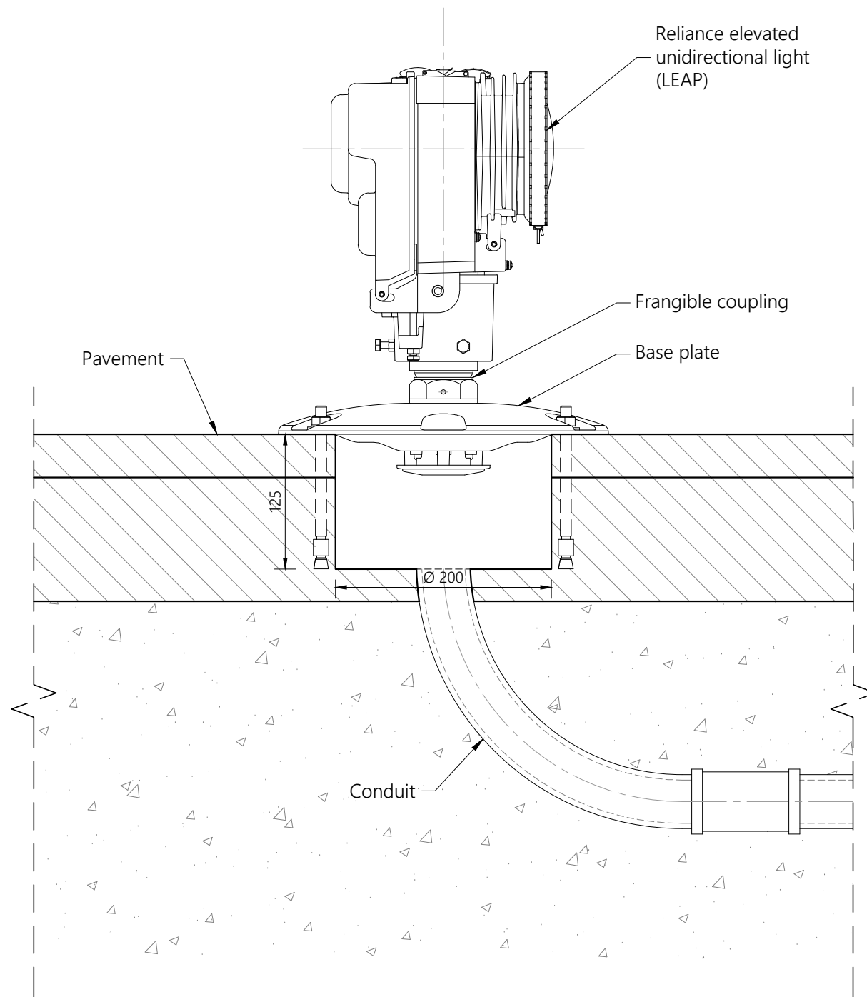
SECTION RELIANCE UNIDIRECTIONAL ELEVATED LIGHT Scale 1/5
