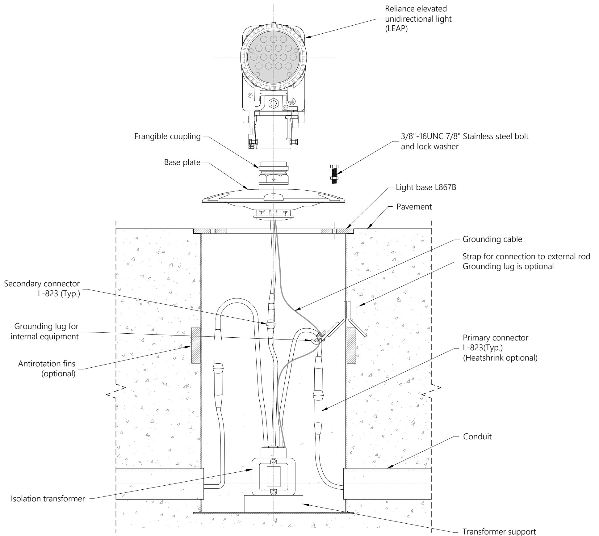
1 PIECE L-867B BASE INSTALLATION RELIANCE UNIDIRECTIONAL ELEVATED LIGHT Scale 1/5
