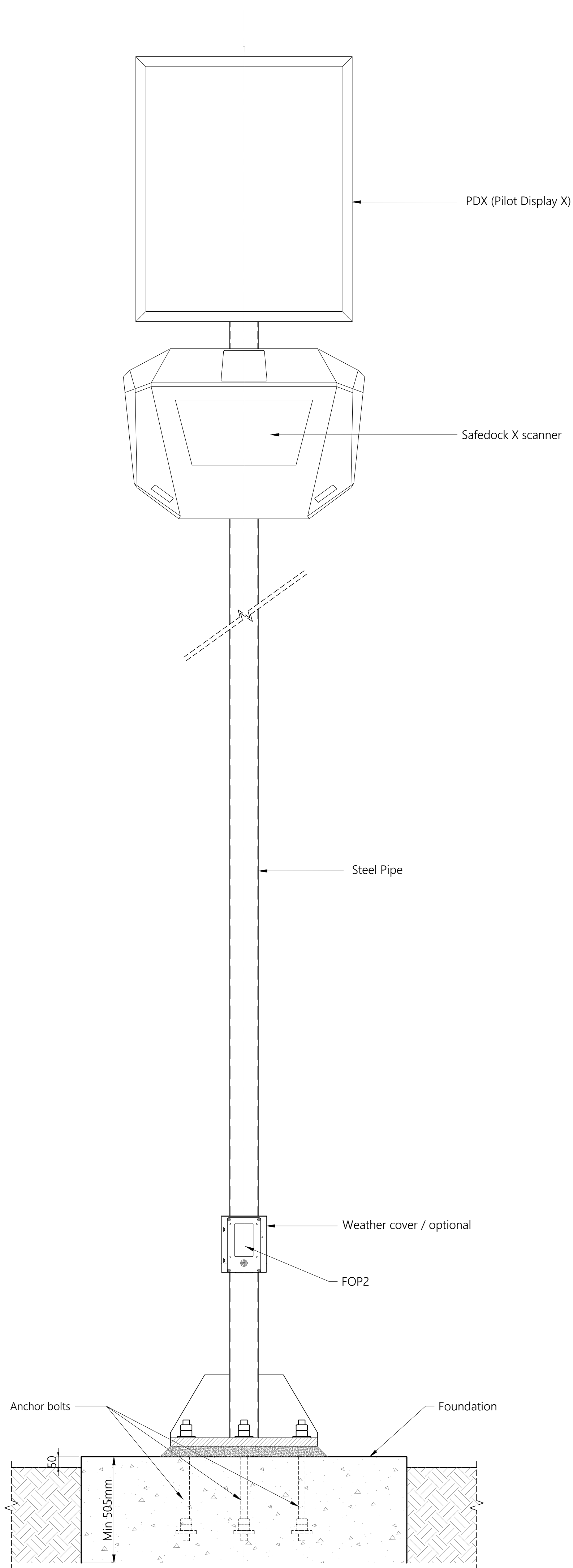
FRONT VIEW A-VDGS SAFEDOCK X - POLE MOUNTING
