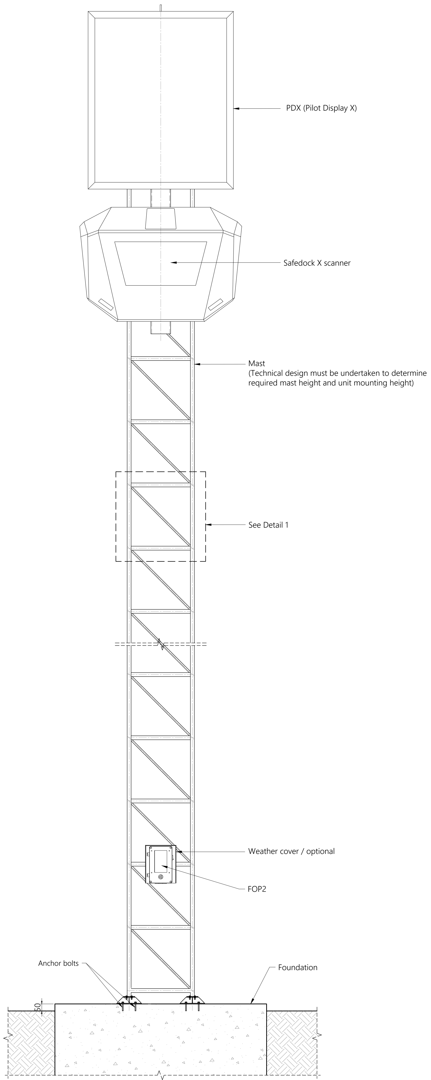
FRONT VIEW A-VDGS SAFEDOCK X - LATTICE MAST MOUNTING
