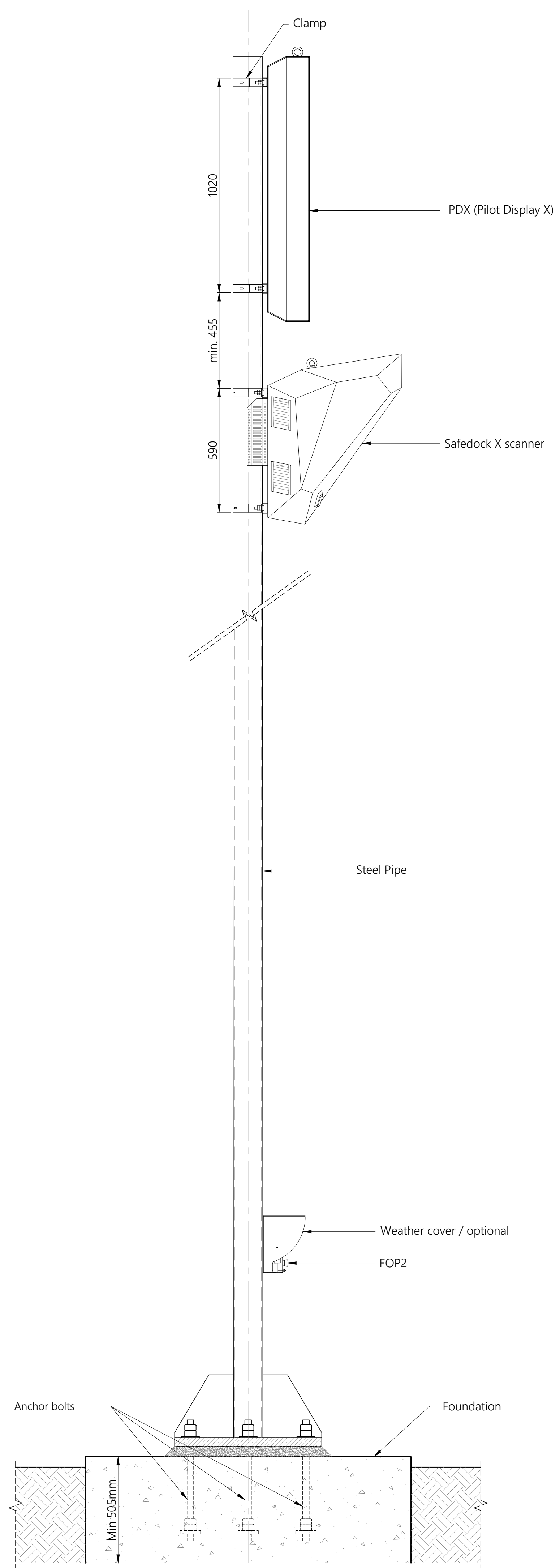
SIDE VIEW A-VDGS SAFEDOCK X - POLE MOUNTING
