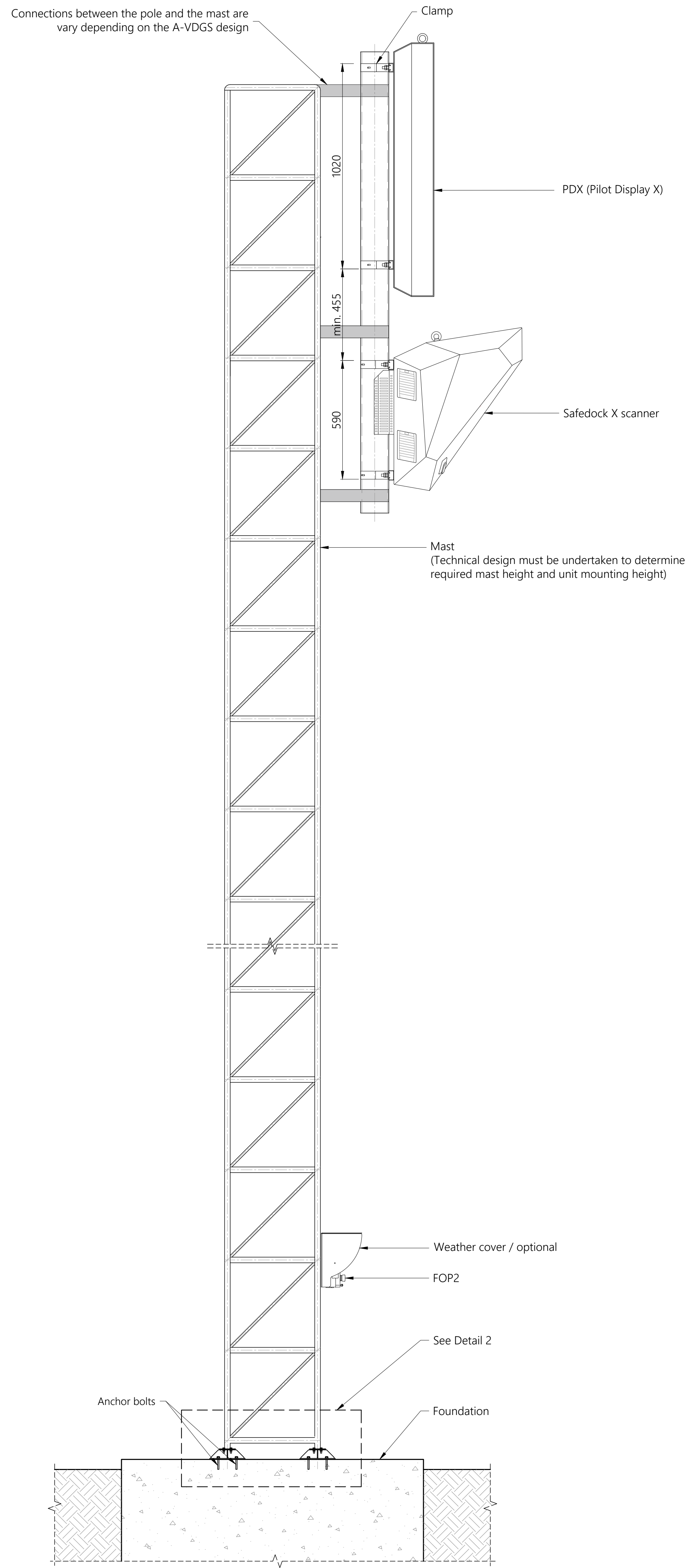
SIDE VIEW A-VDGS SAFEDOCK X - LATTICE MAST MOUNTING
