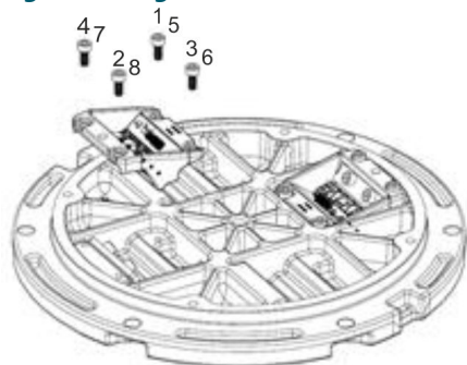
Figure 15: Tighten screws
