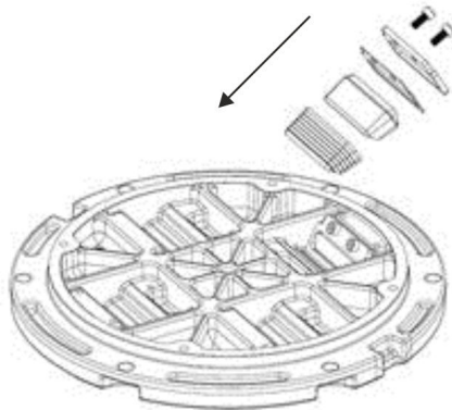
Figure 19: New prism into prism gasket
