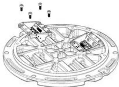
Figure 14: Replacing a light engine
