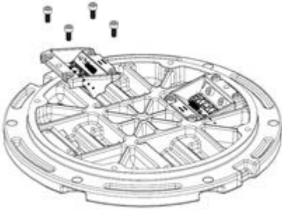
Figure 17: Remove LED board holder
