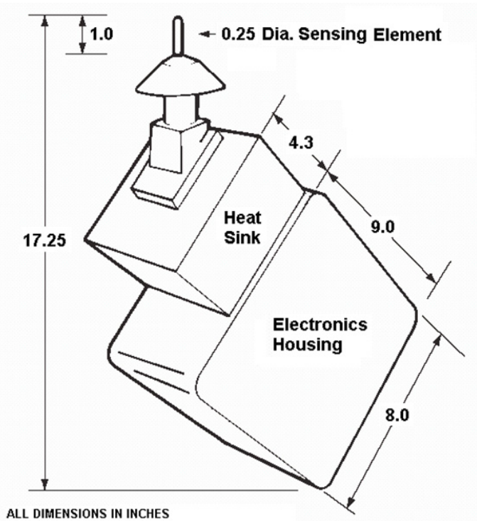
Figure 1. Freezing Rain Sensor Components
