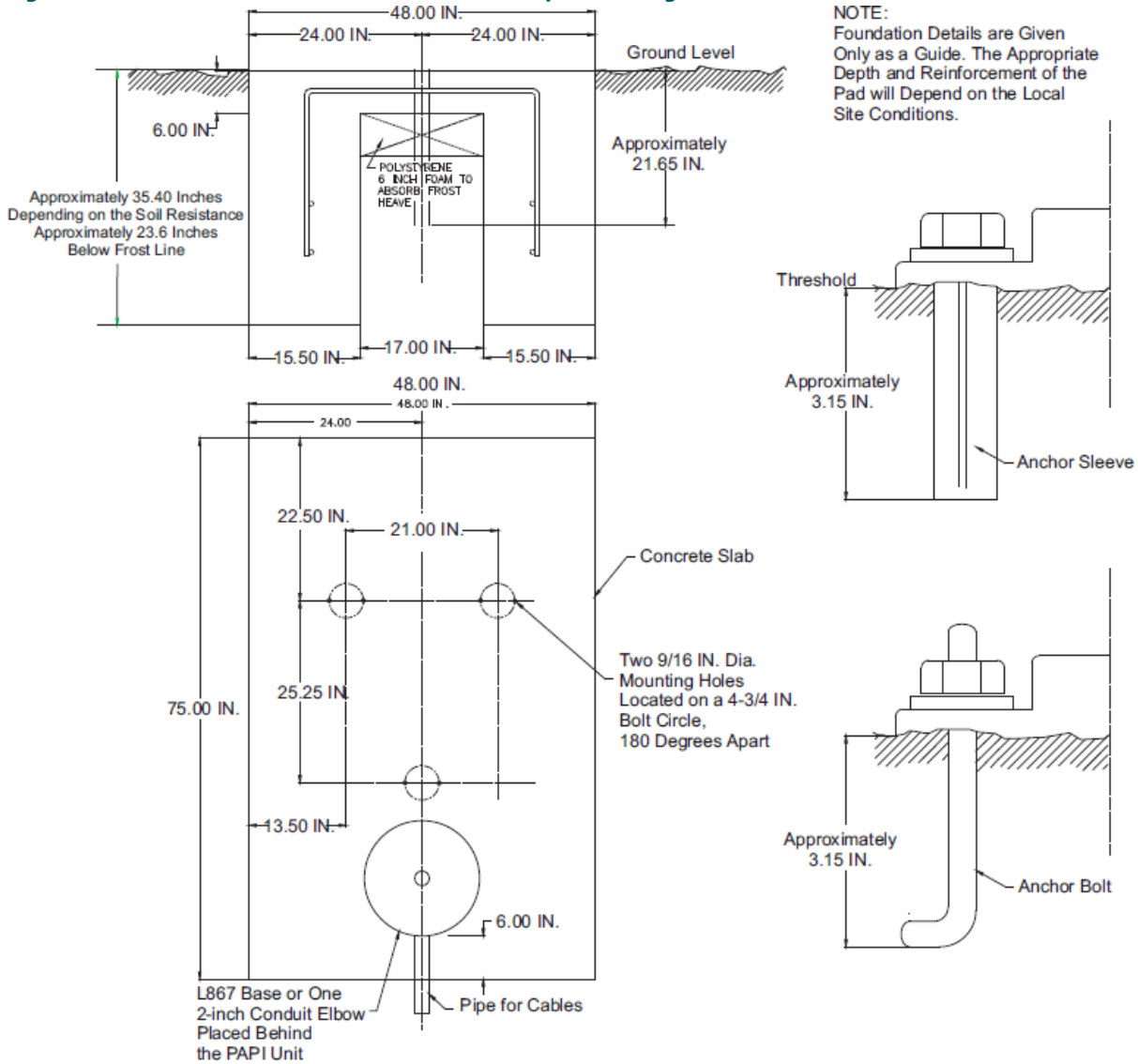
Figure 16: Installation on Concrete Pad (Three-Lamp, Three-Leg PAPI)
