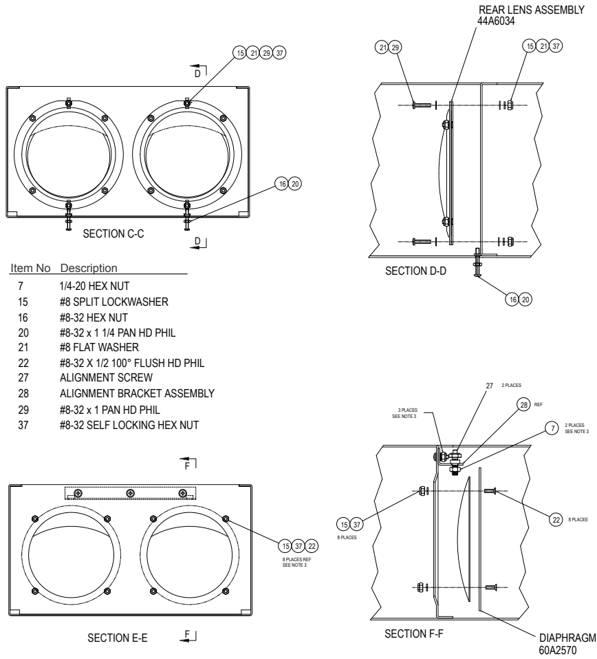
Figure 43: Optical Box Parts Detail C-C, E-E
