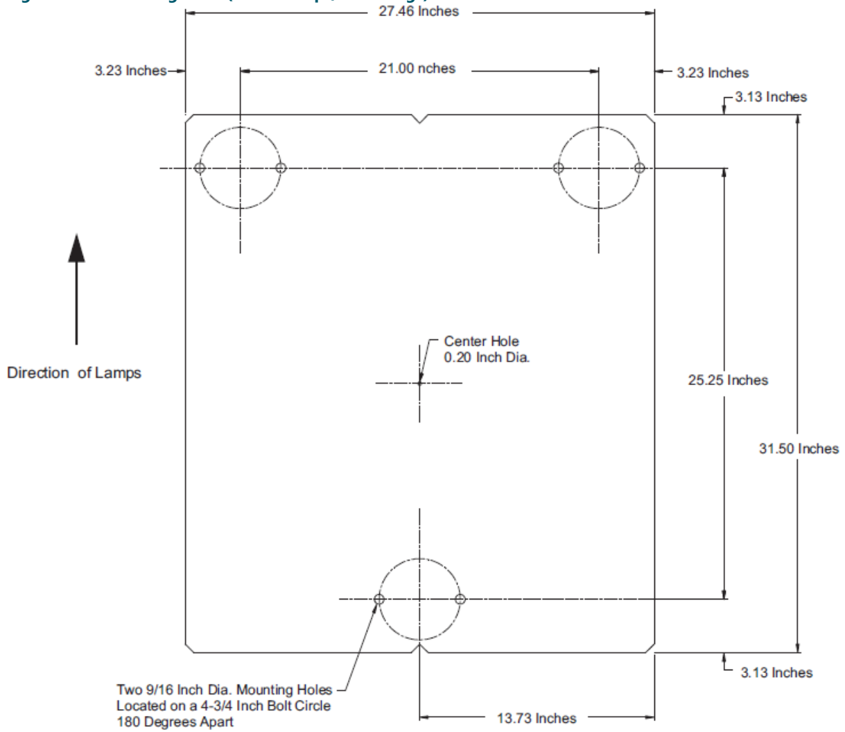
Figure 20: Positioning Plate (Three Lamps/Three Legs)
