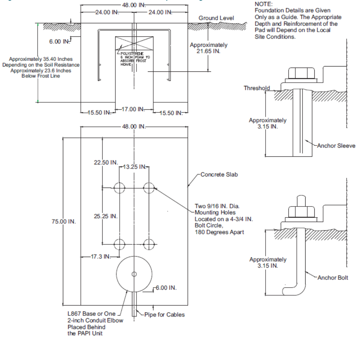
Figure 15: Installation on Concrete Pad (Two-Lamp, Four-Leg PAPI)
