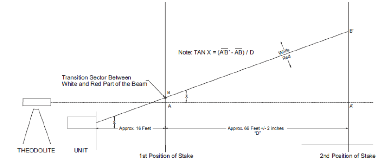
Figure 33: Checking Slope Angles
