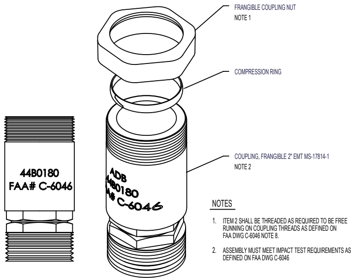
Figure 46: Frangible Coupling 44B0180
