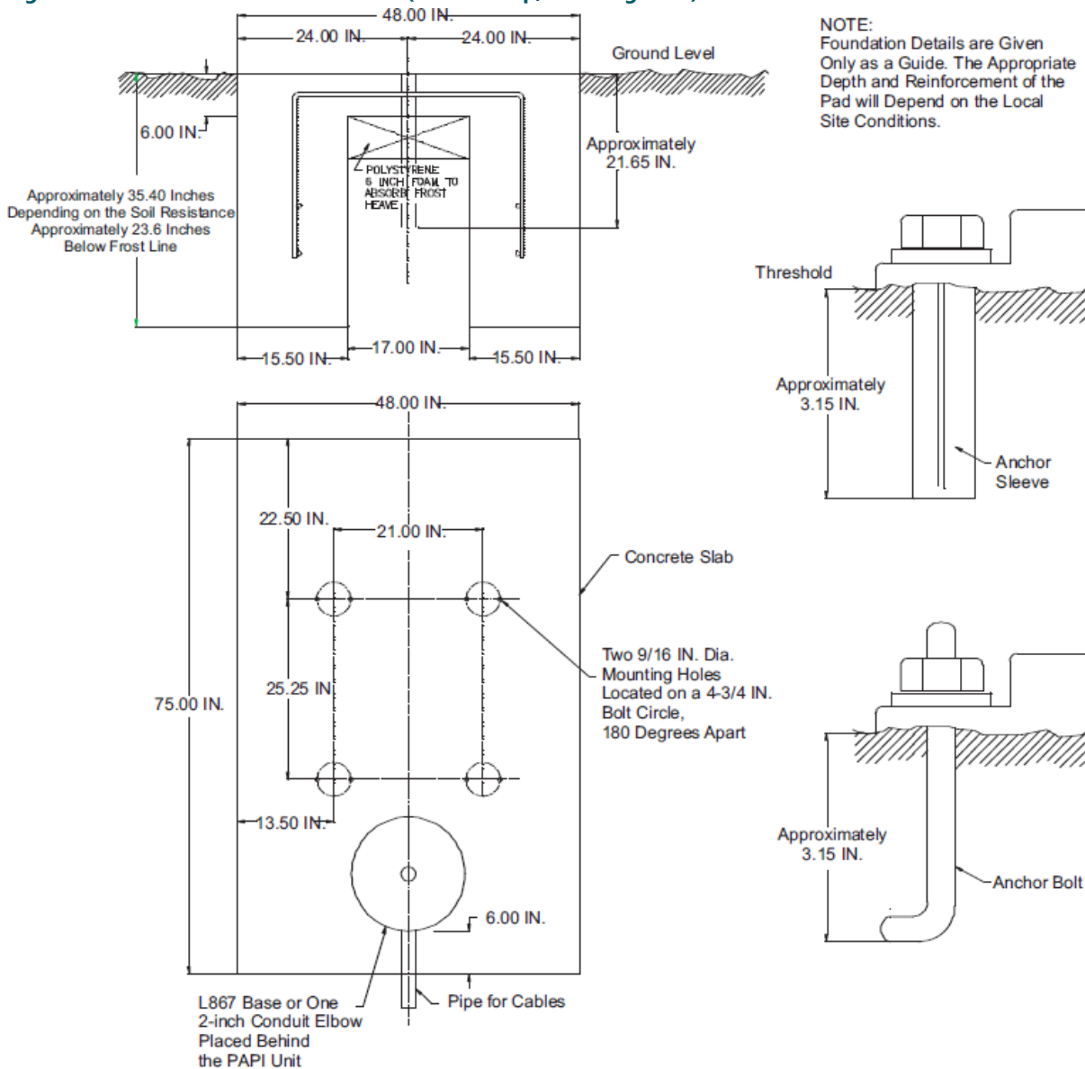
Figure 17: Installation on Concrete Pad (Three-Lamp, Four-Leg PAPI)
