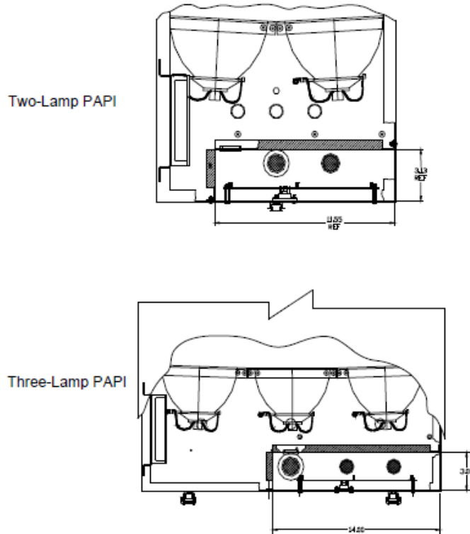
Figure 6: PAPI Light Unit
