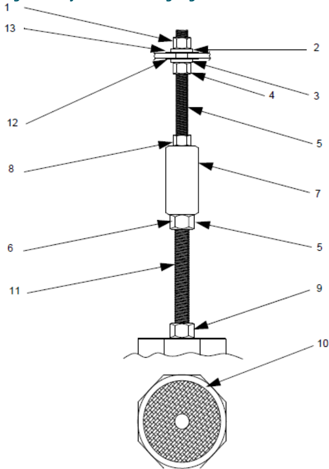
Figure 7: Adjustable Mounting Legs
