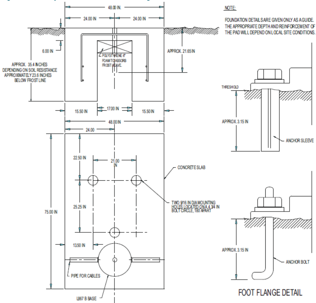
Figure 38: PAPI Style B Master and Slave Three-leg Foundation Detail
