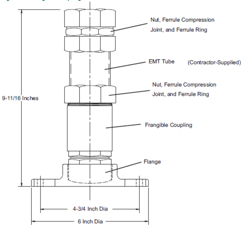
Figure 22: Frangible Coupling
