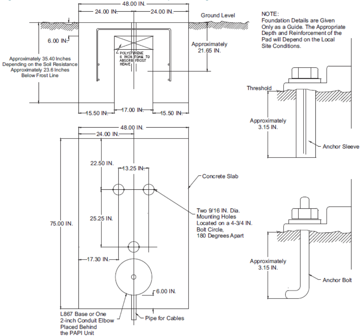
Figure 14: Installation on Concrete Pad (Two-Lamp, Three-Leg PAPI)
