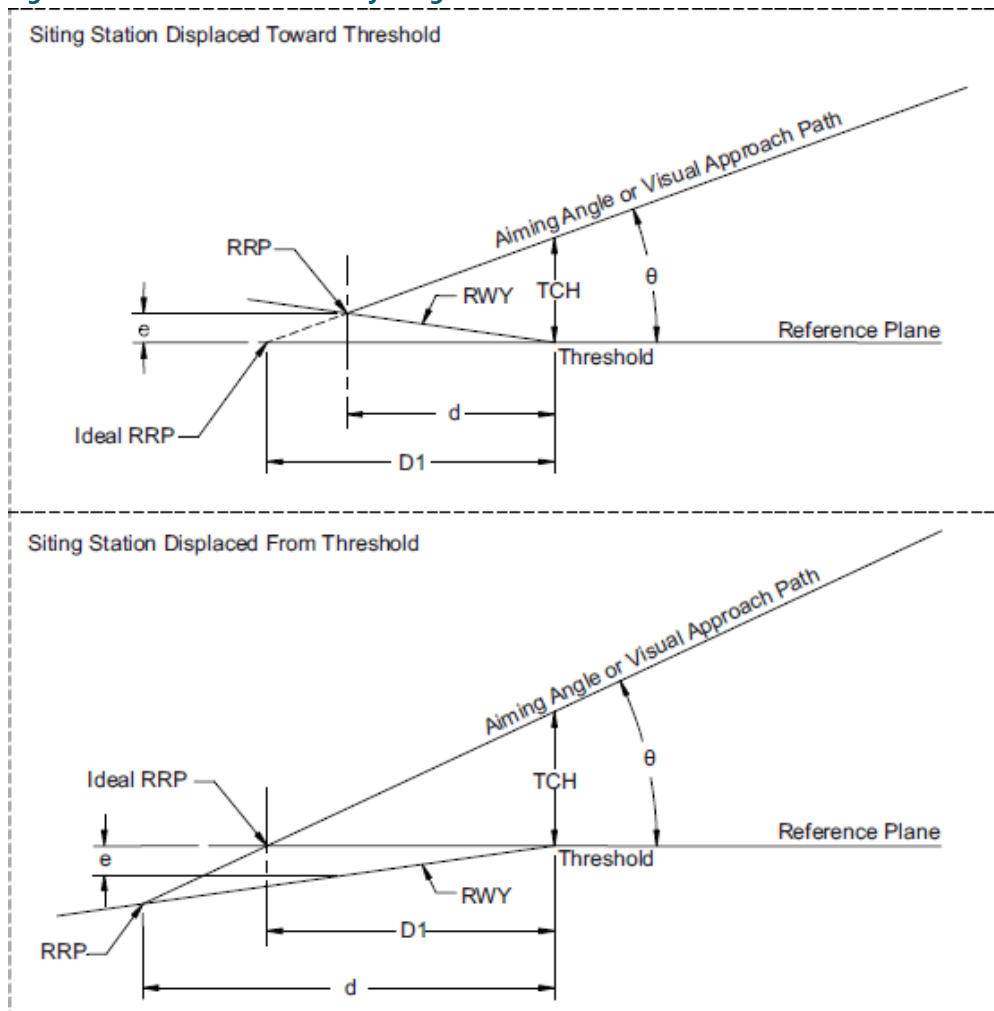
Figure 12: Correction for Runway Longitudinal Gradient
