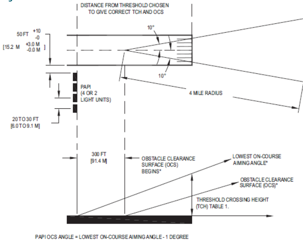
Figure 3: PAPI Obstacle Clearance Surface
