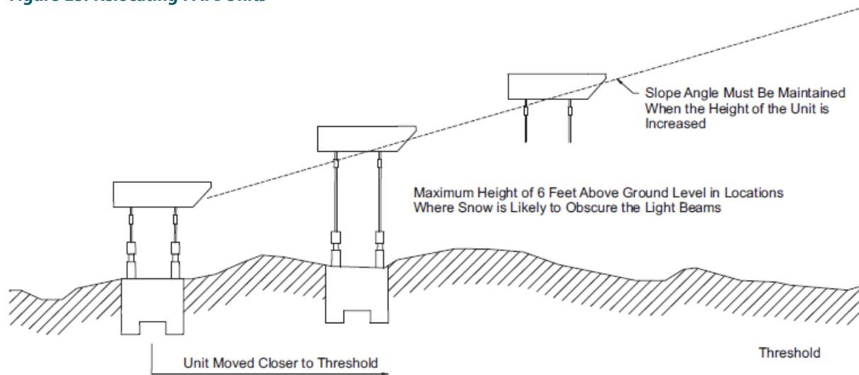
Figure 13: Relocating PAPI Units
