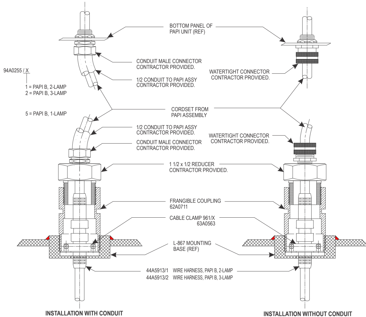
Figure 47: Field Splice Kit 94A0255/X
