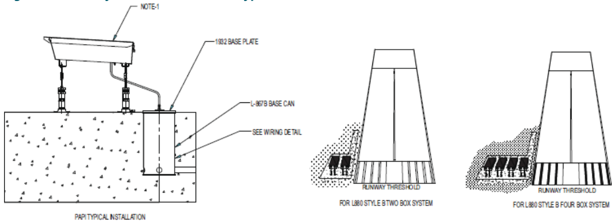
Figure 37: PAPI Style B Master and Slave Typical Installation
