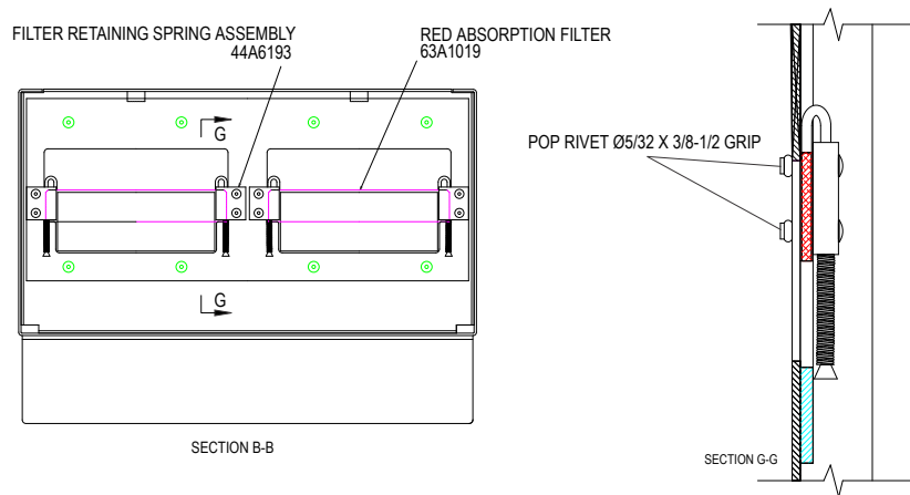
Figure 42: Optical Box Part Detail B-B
