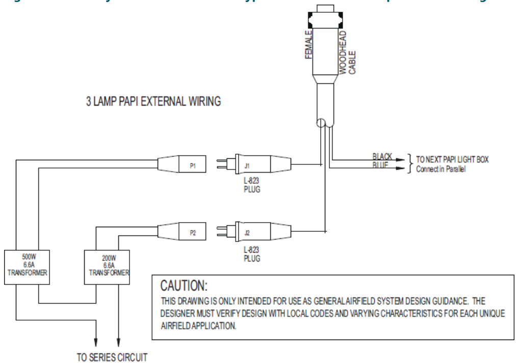
Figure 35: PAPI Style B Master and Slave Typical Installation 3-Lamp External Wiring
