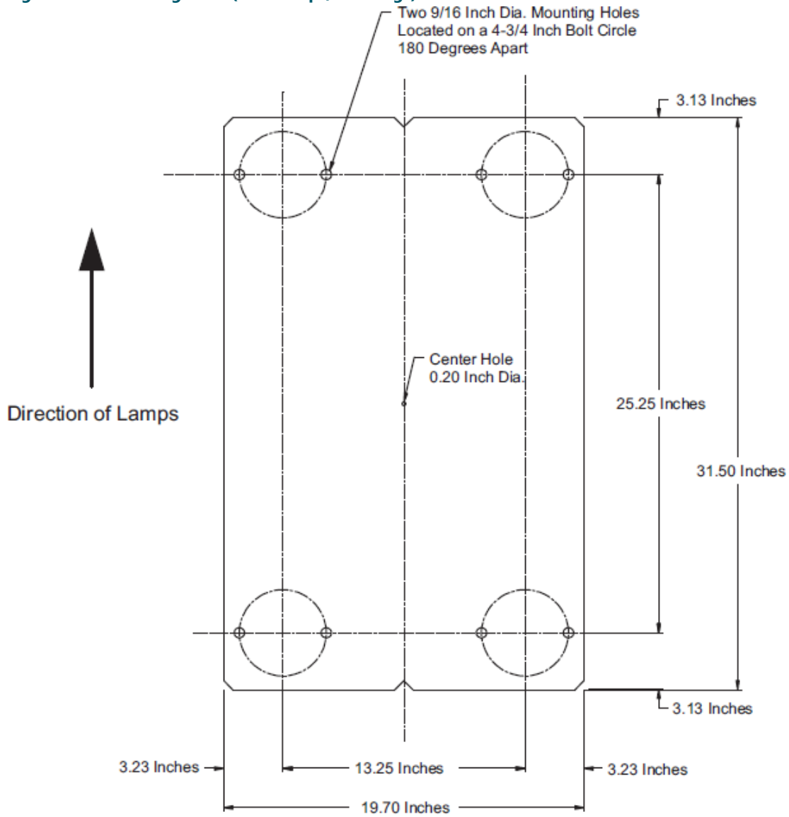
Figure 19: Positioning Plate (Two Lamps/Four Legs)
