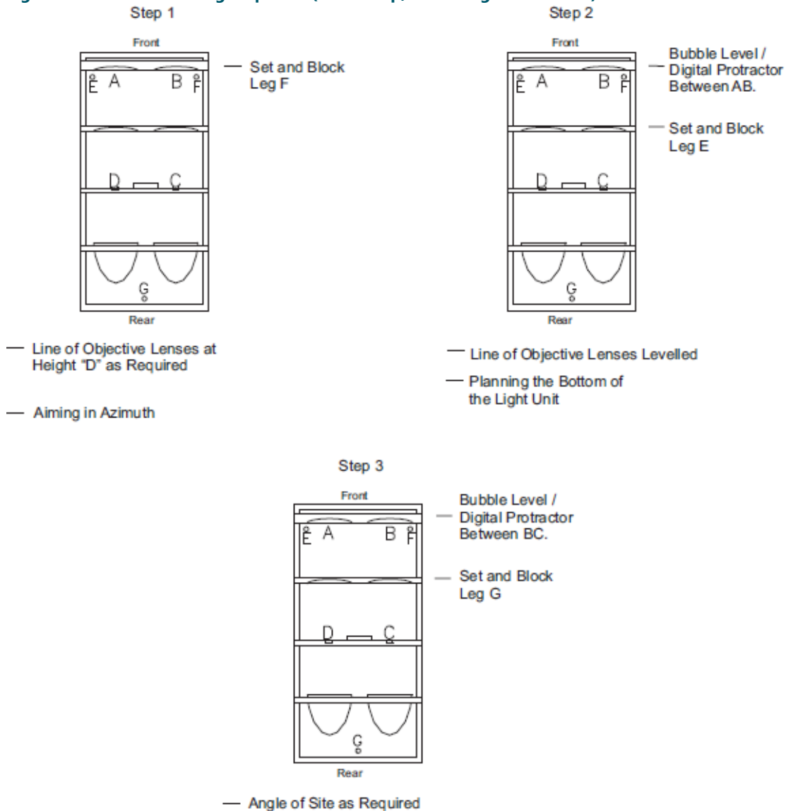
Figure 24: Elevation Setting Sequence (Two-Lamp, Three-Leg PAPI Shown)
