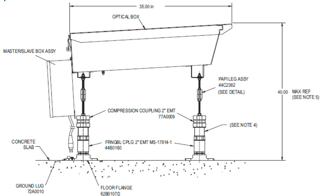
Figure 44: Optical Box Side View
