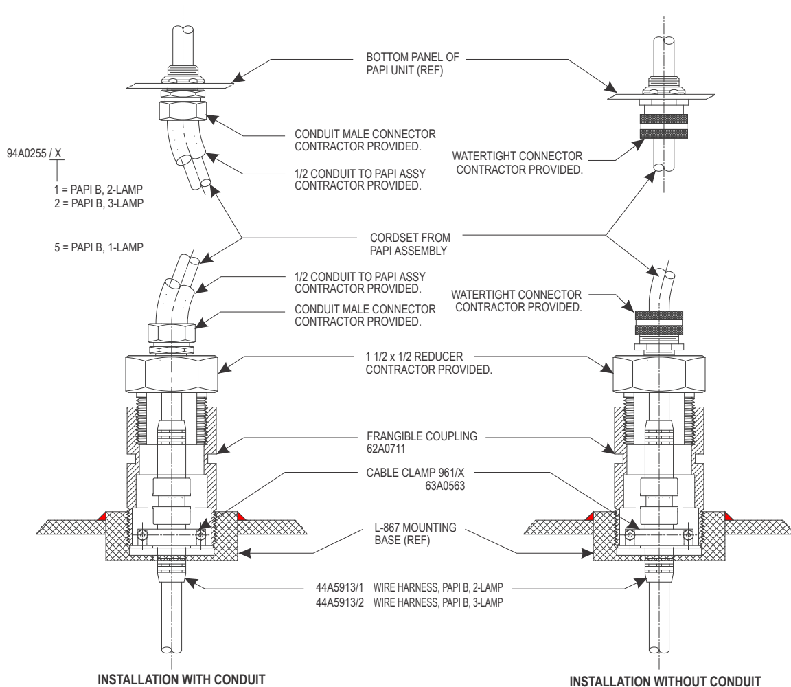
Figure 32: PAPI External Connections (Two- and Three-Lamp)
