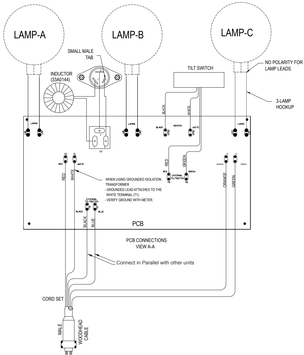
Figure 40: Two- and Three-Lamp PAPI Optical Box Internal Wiring
