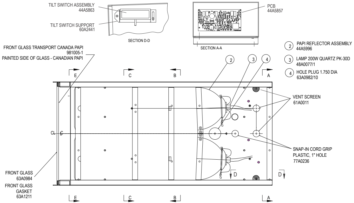
Figure 41: Optical Box Parts and Details
