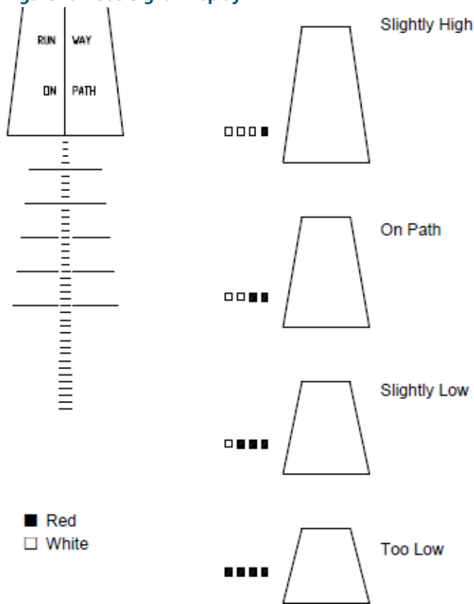
Figure 4: L-880 Signal Display
