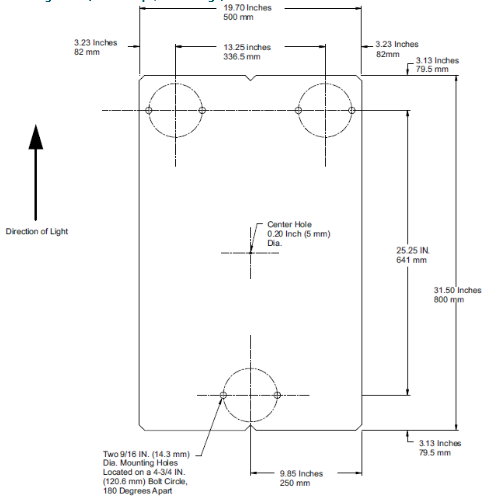
Figure 18: Positioning Plate (Two Lamps/Three Legs)
