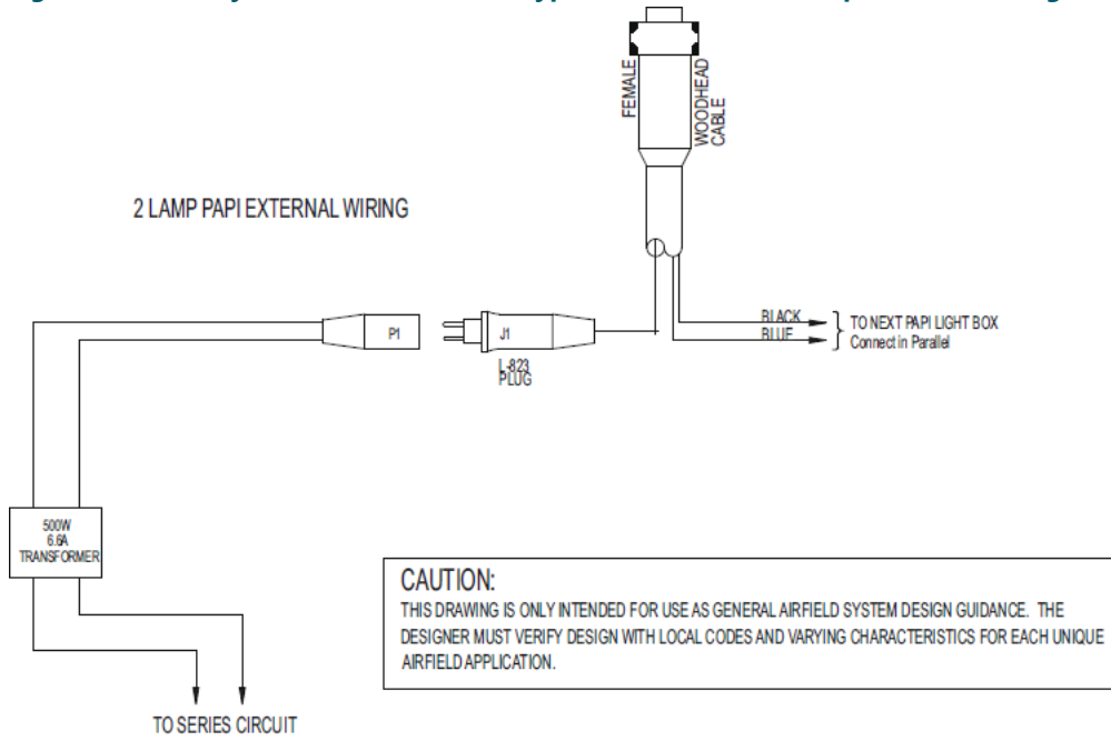
Figure 37: PAPI Style B Master and Slave Typical Installation
