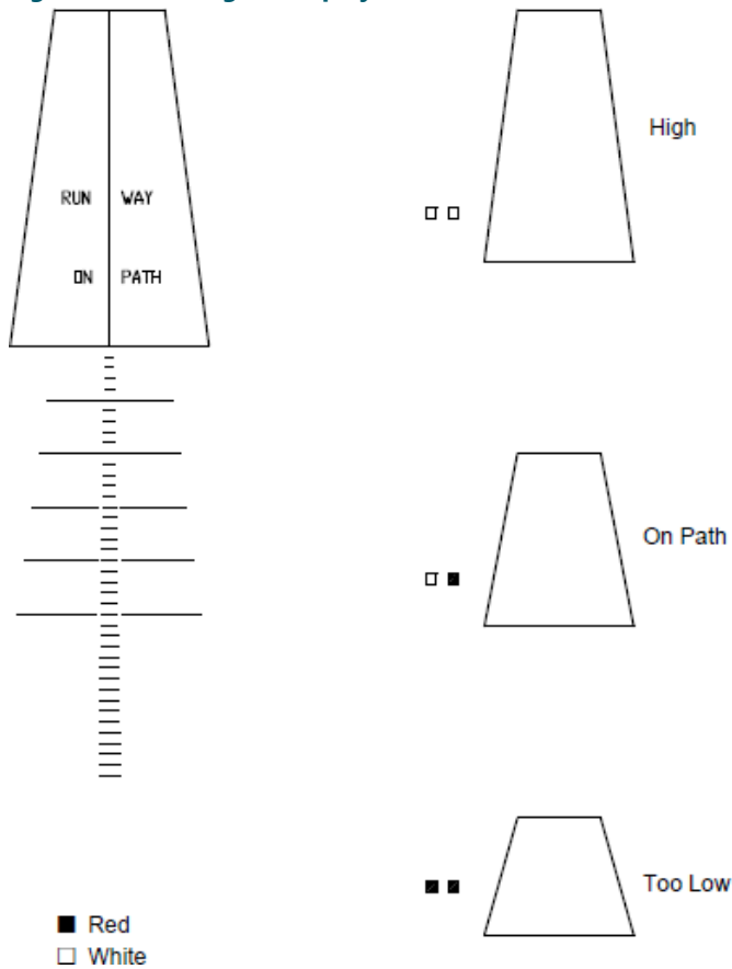
Figure 5: L-881 Signal Display
