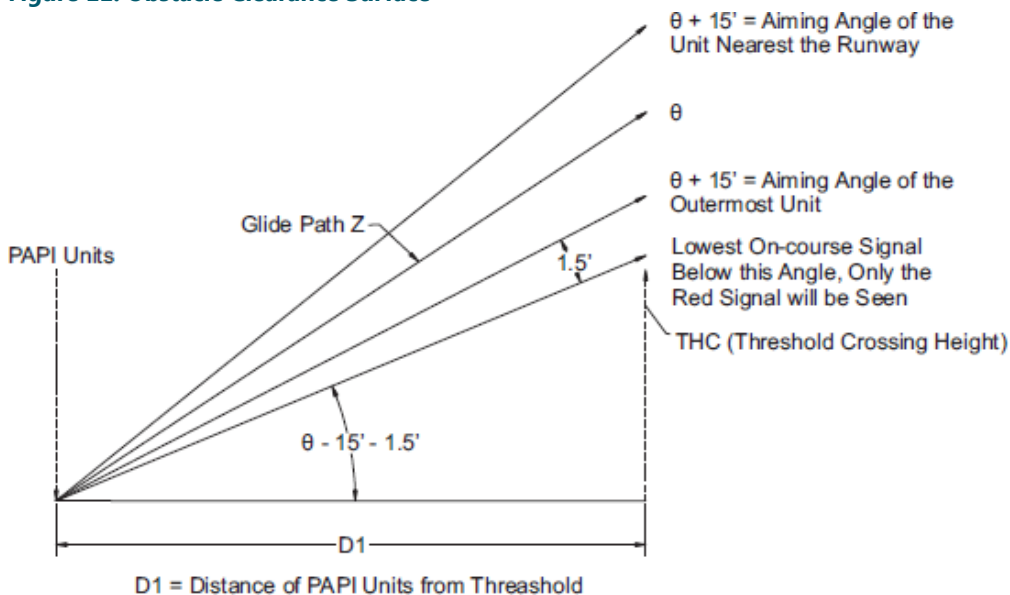
Figure 11: Obstacle Clearance Surface
