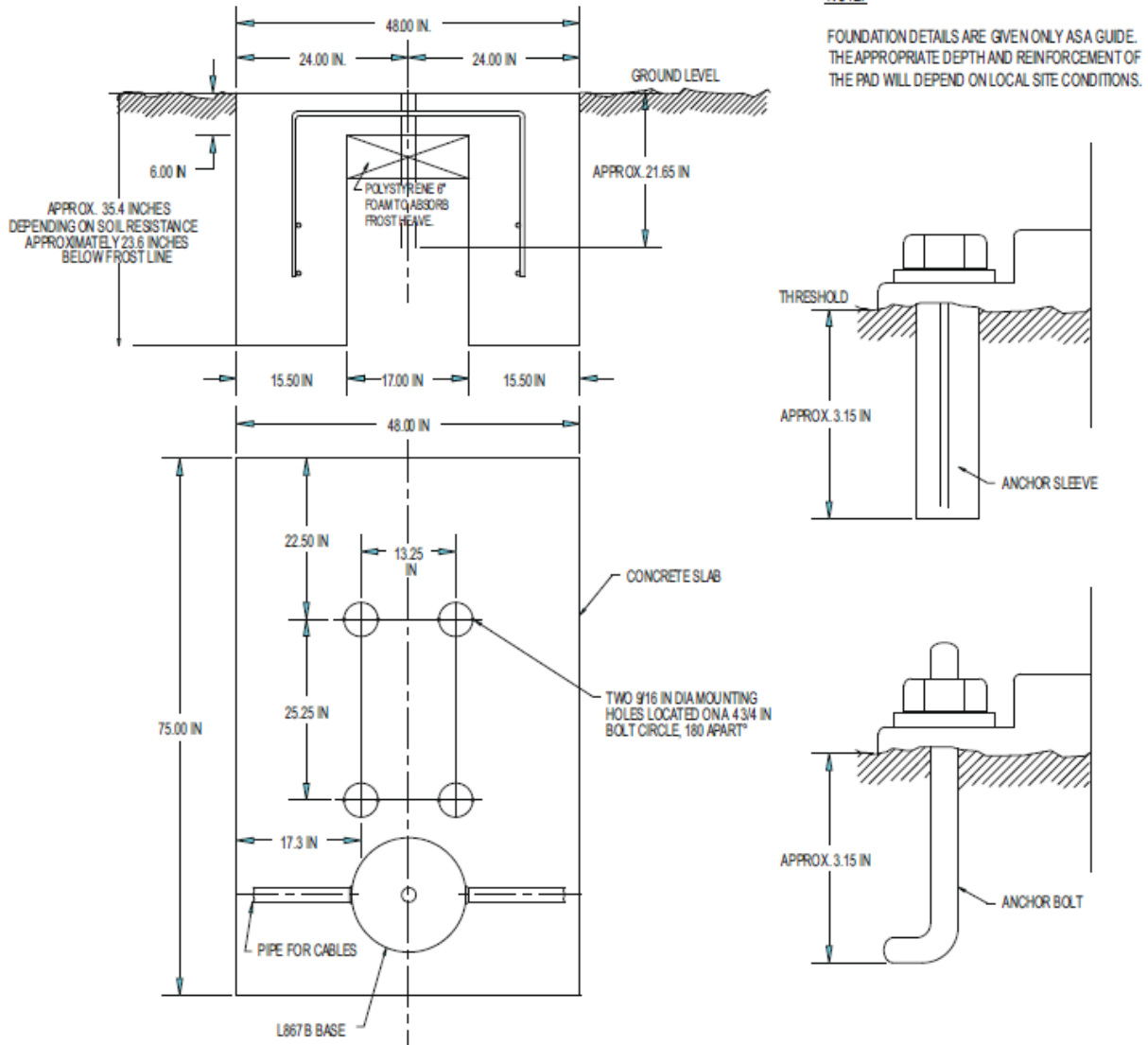
Figure 39: PAPI Style B Master and Slave Four-leg Foundation Detail
