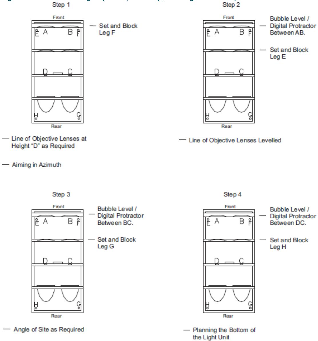
Figure 23: Elevation Setting Sequence (Two-Lamp, Four-Leg PAPI Shown)
