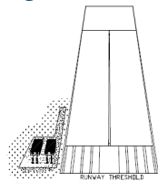
Figure 2: L-881 Two-Box PAPI System
