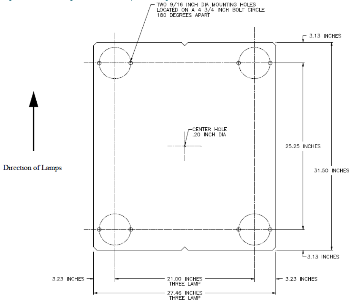
Figure 21: Positioning Plate (Three Lamps/Four Legs)
