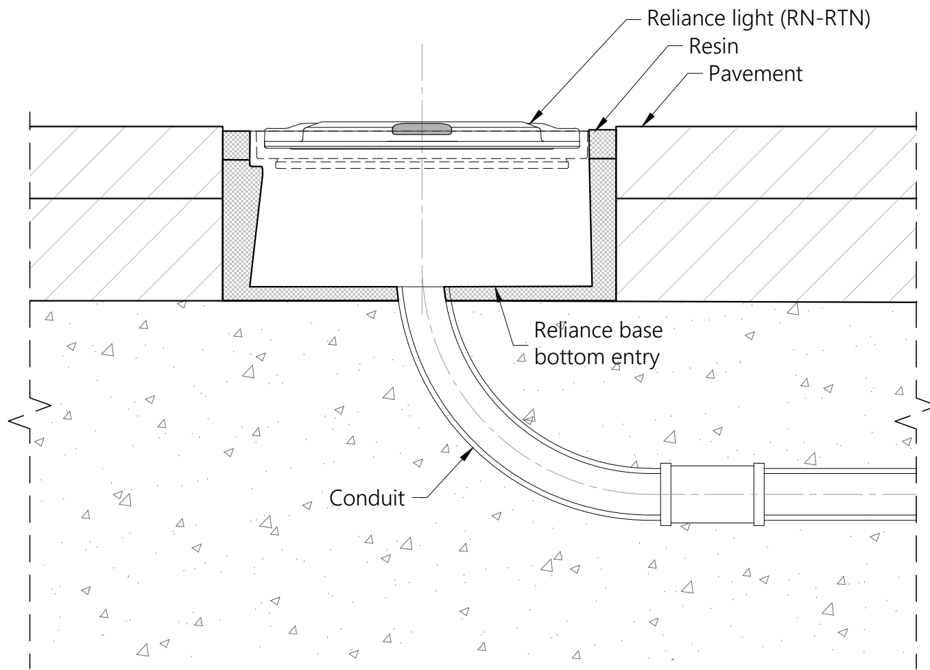
SECTION RELIANCE INSET 12" BIDIRECTIONAL LIGHT (3 Windows) Scale 1/5
