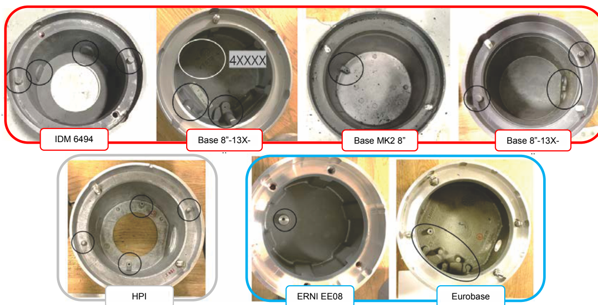
Figure 56: Shallow bases
