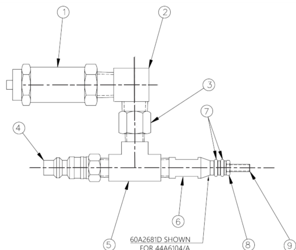
Figure 45: Pressure test fitting tool
