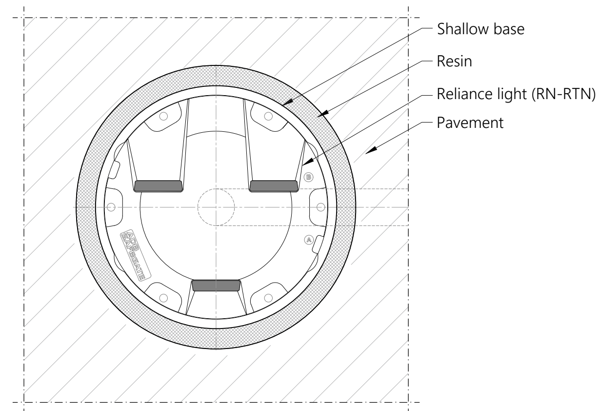
TOP VIEW RELIANCE INSET 12" BIDIRECTIONAL LIGHT (3 Windows) Scale 1/5
