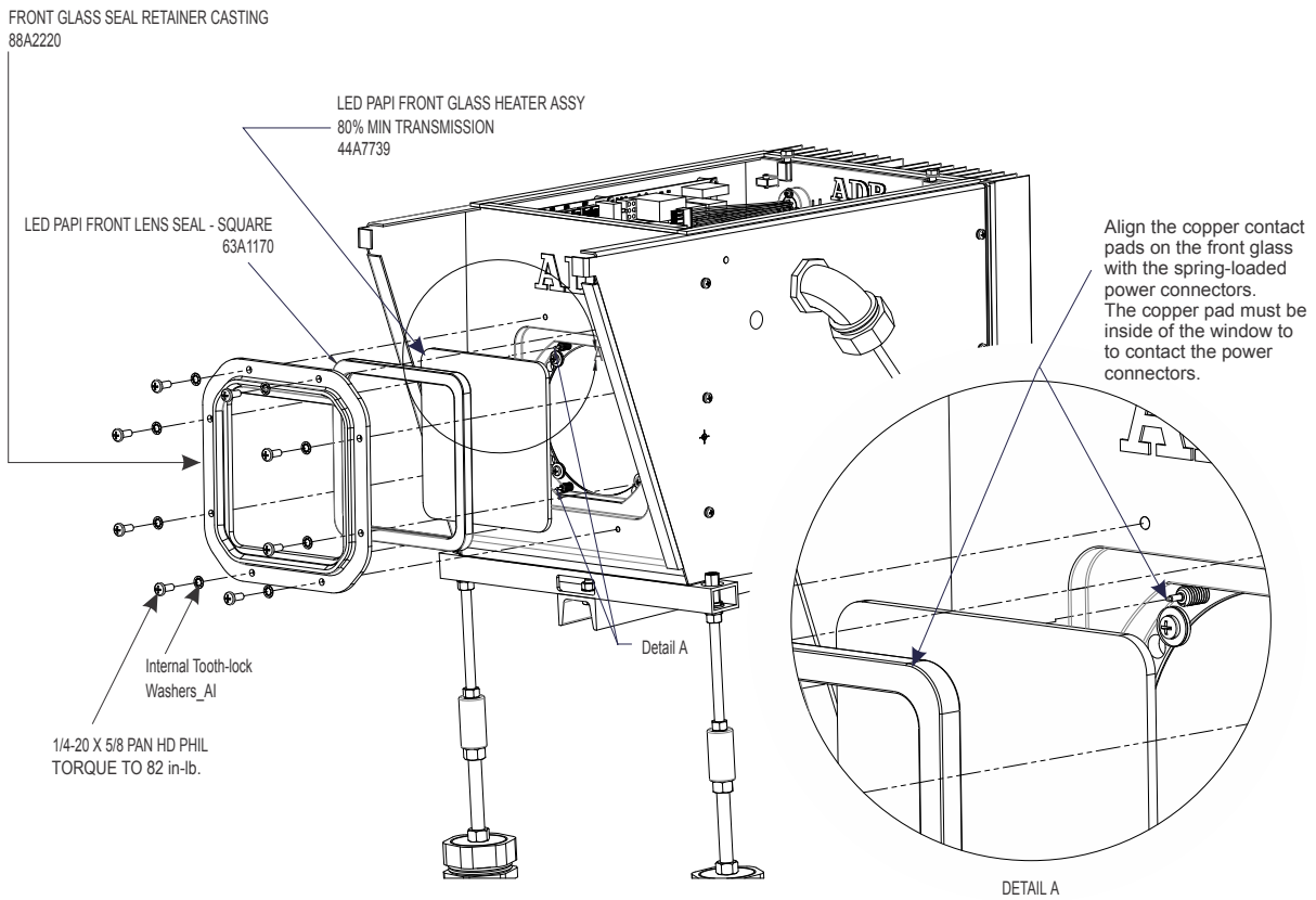
Figure 10: Front Glass Replacement
