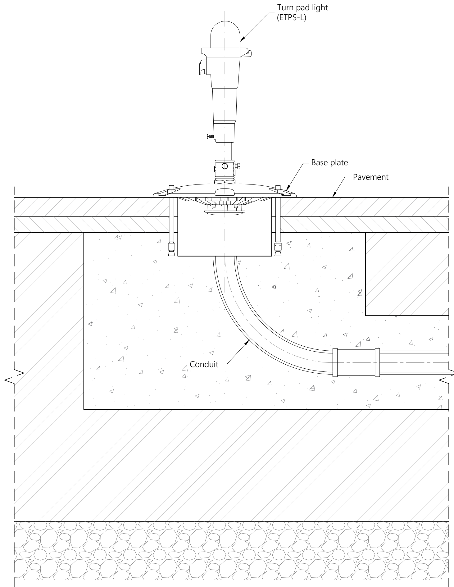
○ SECTION RELIANCE TURNPAD OMNIDIRECTIONAL ELEVATED Scale 1/5
