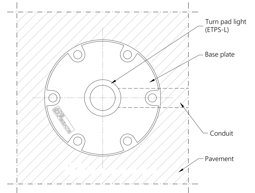
○ TOP VIEW RELIANCE TURNPAD OMNIDIRECTIONAL ELEVATED Scale 1/5
