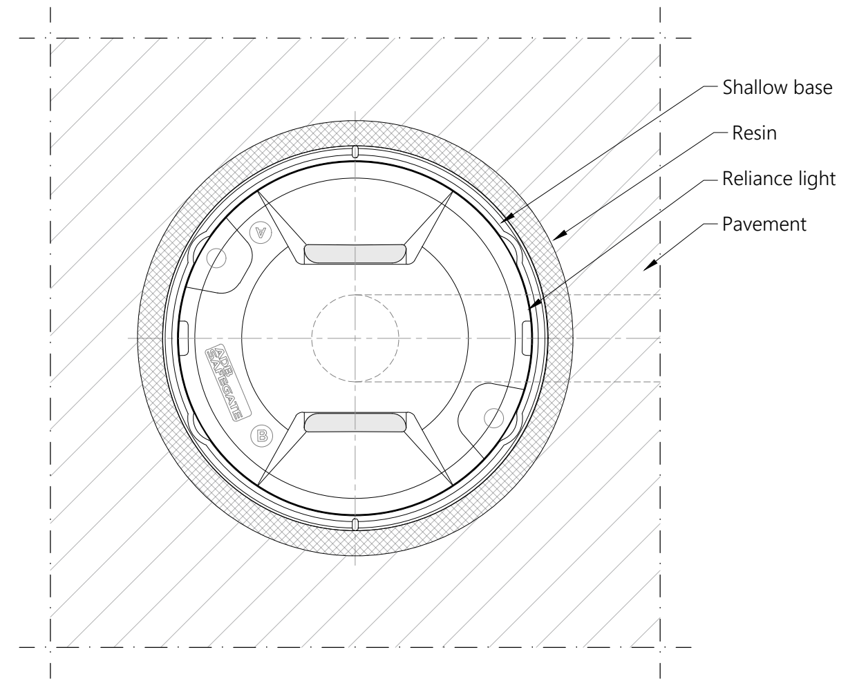
TOP VIEW RELIANCE INSET 8" BIDIRECTIONAL LIGHT Scale 1/3
