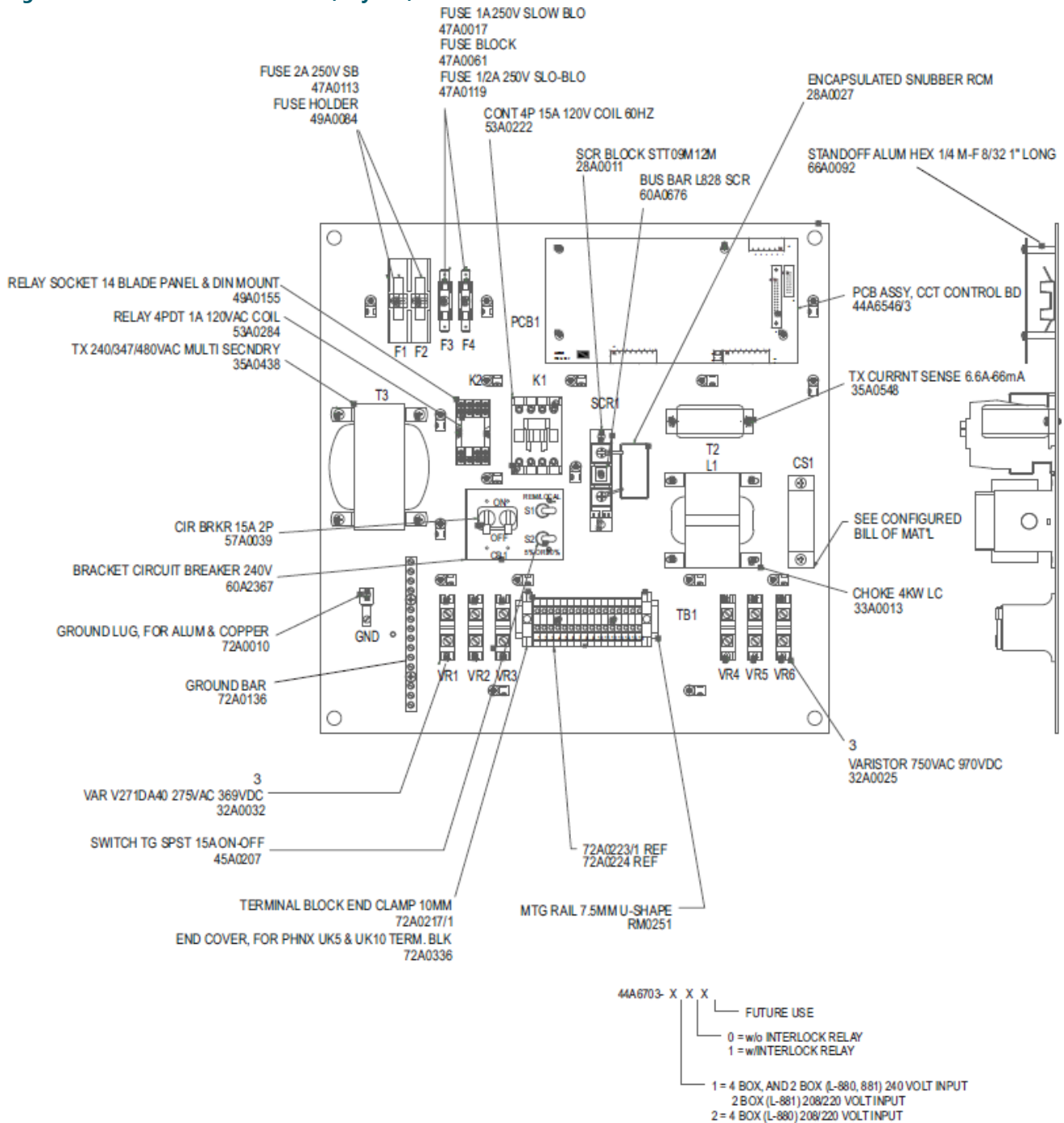
Figure 40: Power Control Unit Panel, Style A, 44A6703
