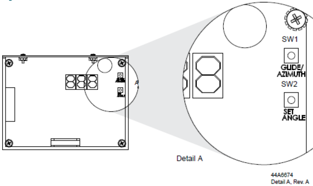
Figure 17: Control Board Pushbuttons
