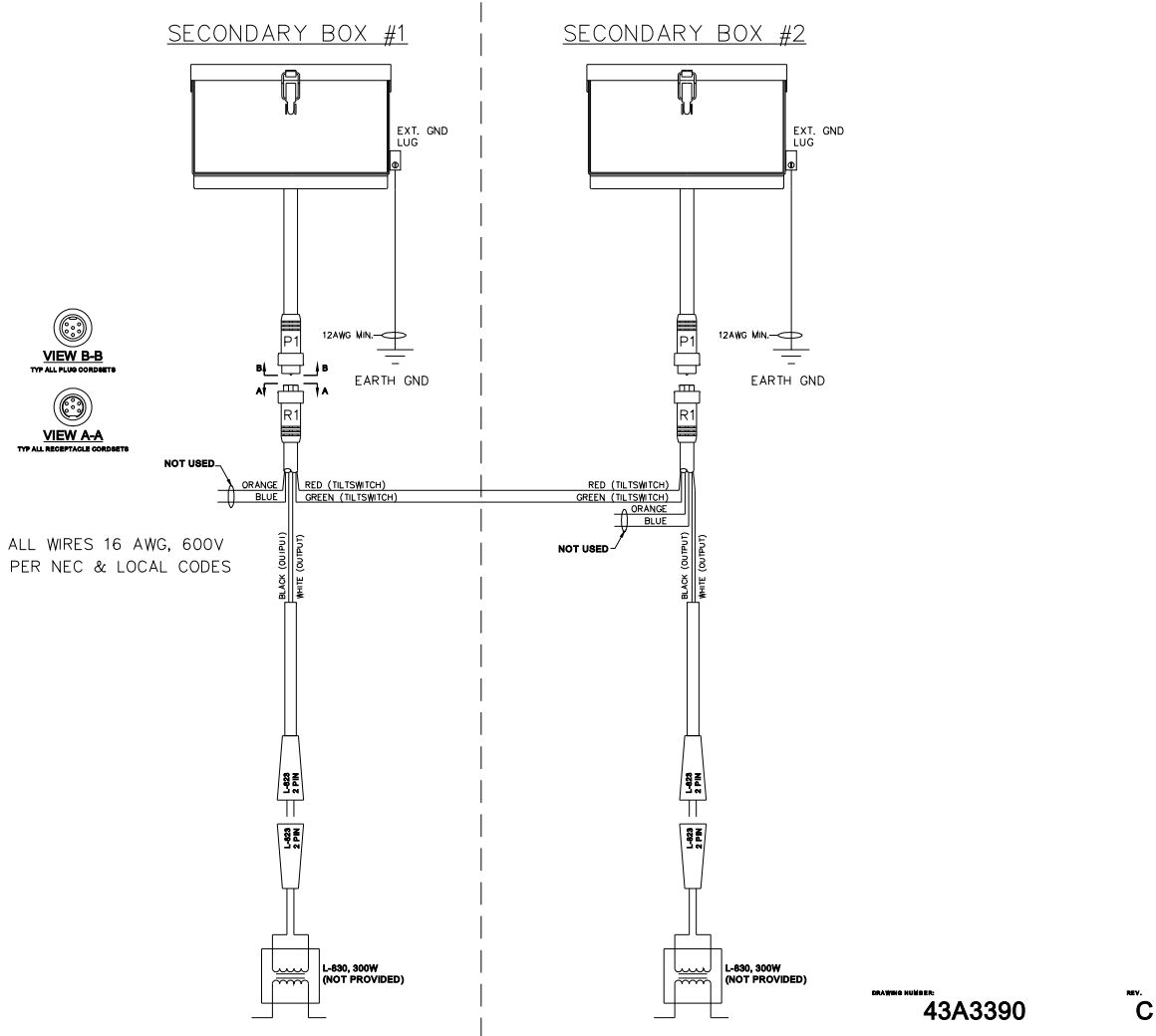
Figure 29: External Wiring, Single Channel PAPI Style B, L-881 (2 Box) System
