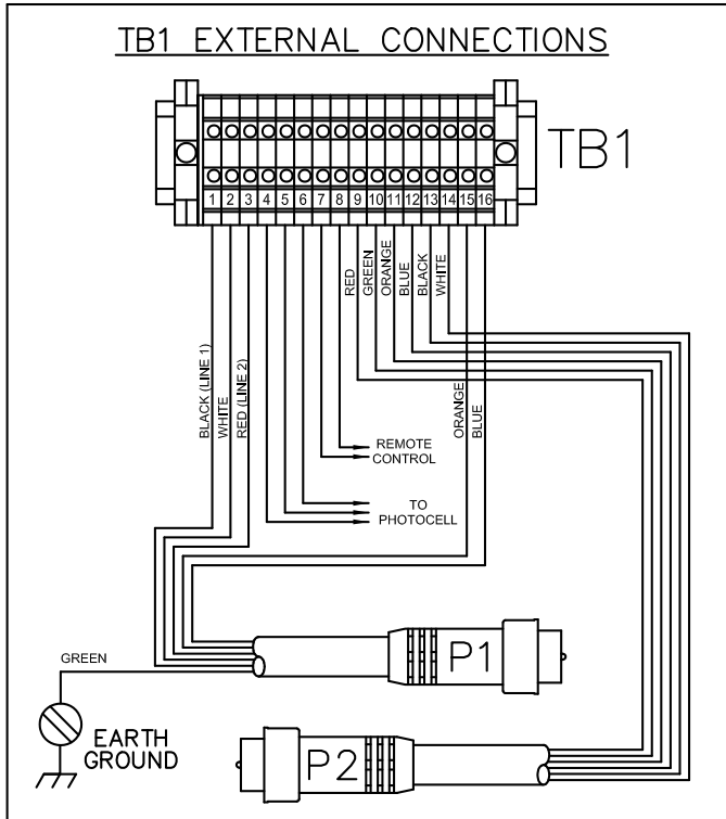
Figure 32: TB1 External Connections
