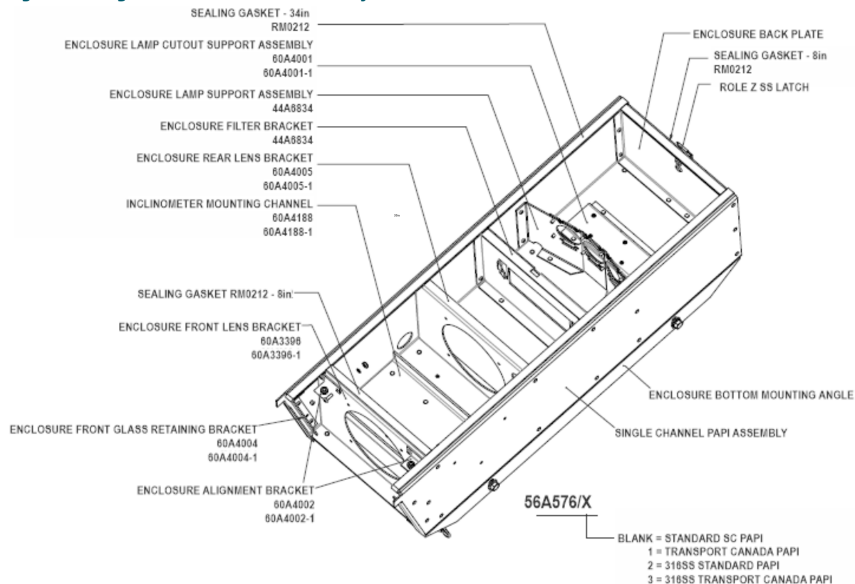
Figure 20: Single Channel PAPI Box Assembly
