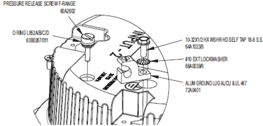
Figure 1: Pressure Release Screw and Ground Lug
