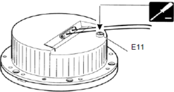
Figure 10: Pressure Release Screw
