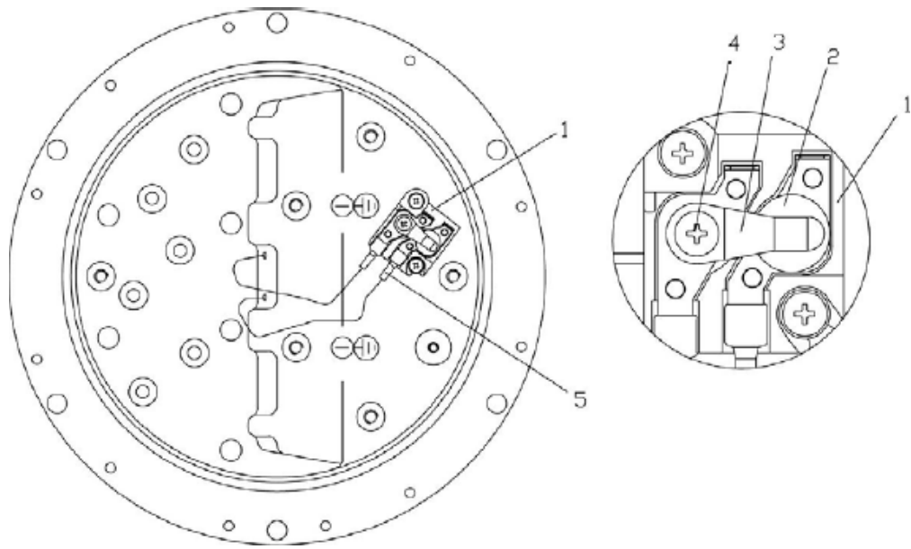
Figure 15: Film Disc Cutout Assembly and Optical Unit
