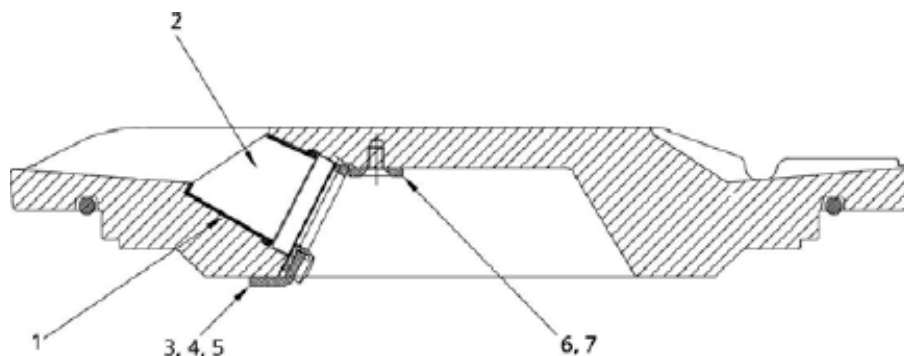
Figure 17: Replacing L-850E Prism
