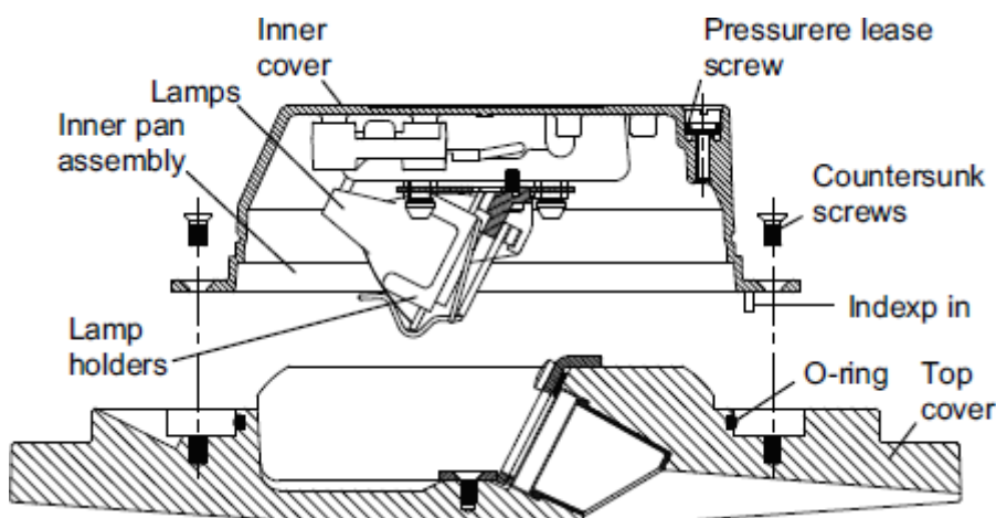
Figure 19: L-850D/E Inset Light Fixture (L-850D – FAA shown)
