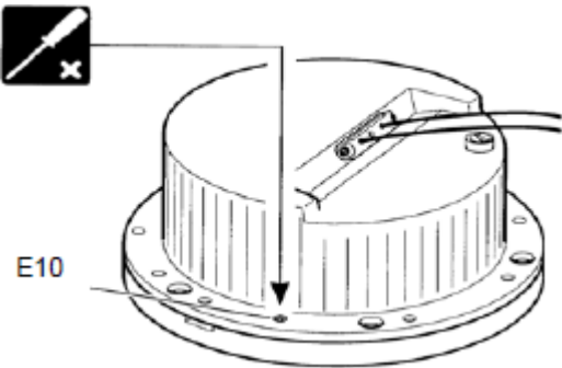
Figure 11: Removing Screws
