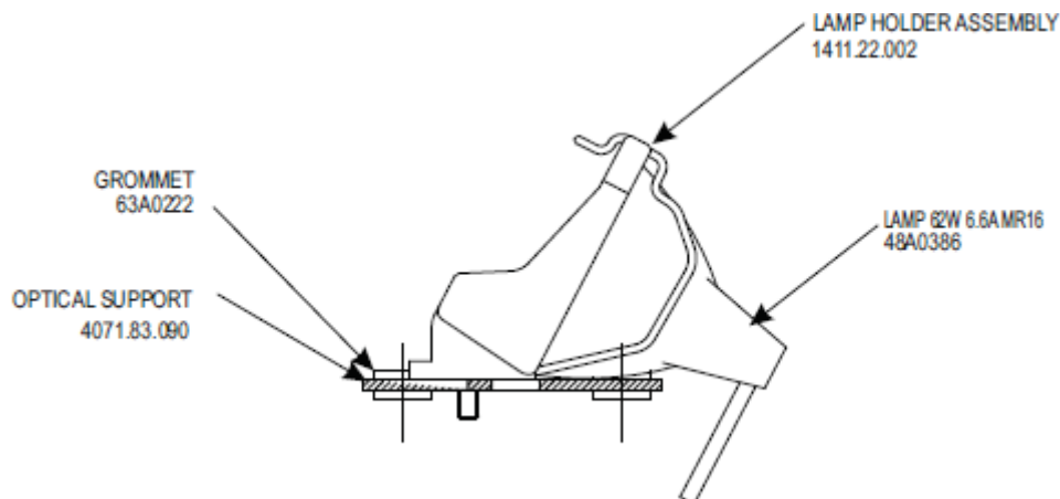
Figure 26: Optical Support Assembly - side view
