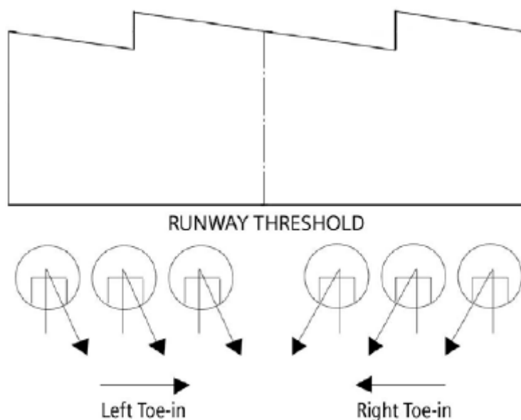
Figure 3: L-850D/E Toe-In Coding
