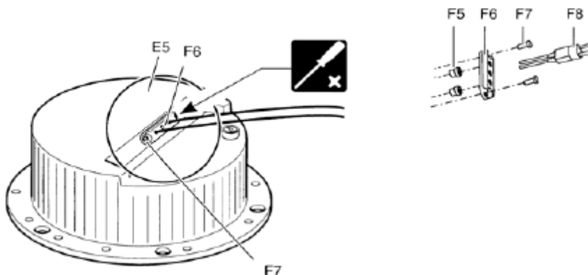
Figure 18: L-823 Cordset
