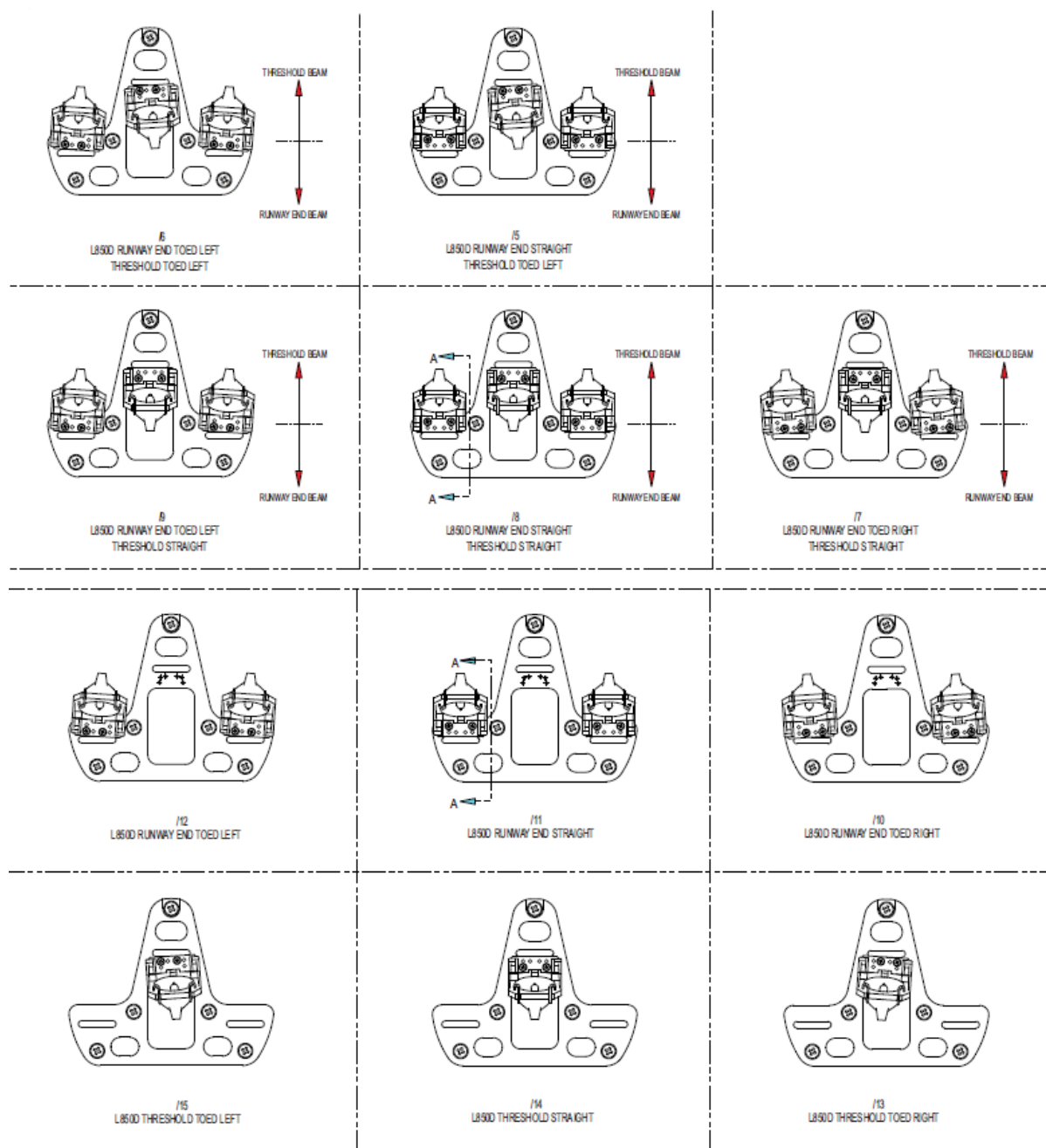
Figure 25: Optical Support Assemblies
