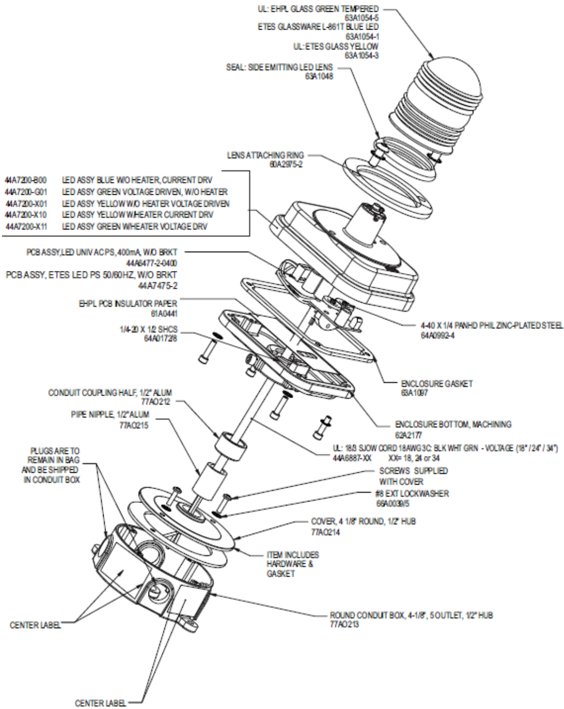
Figure 12: Assembly
