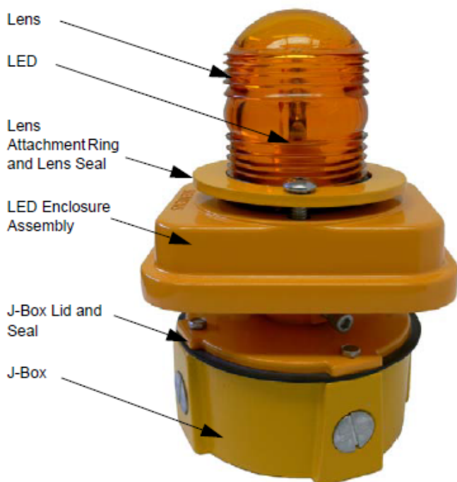
Figure 1: EHP-L Assembly (direct J-Box mounting shown)
