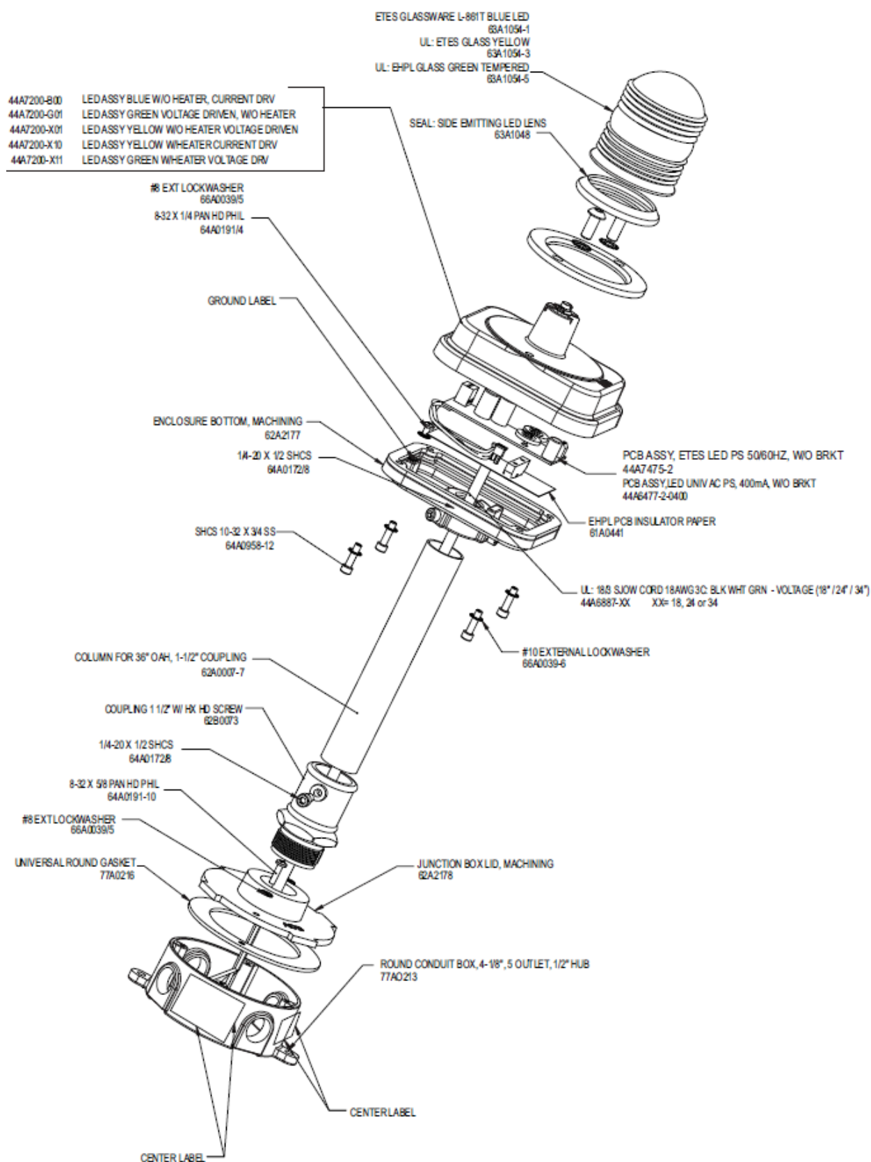
Figure 11: EHP-L Assembly
