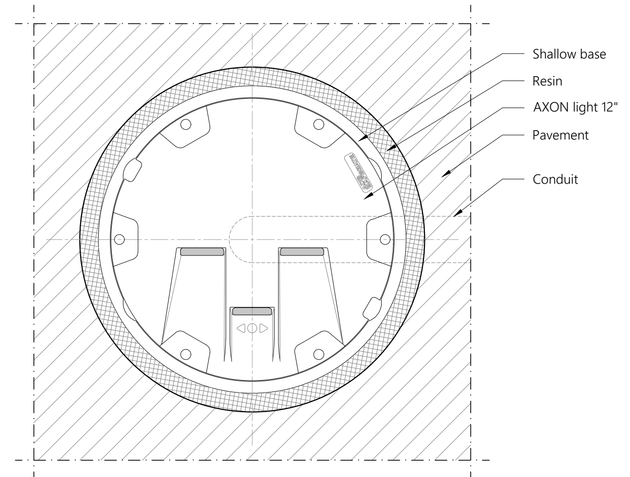
TOP VIEW AXON INSET 12" UNIDIRECTIONAL LIGHT (3 windows) Scale 1/4
