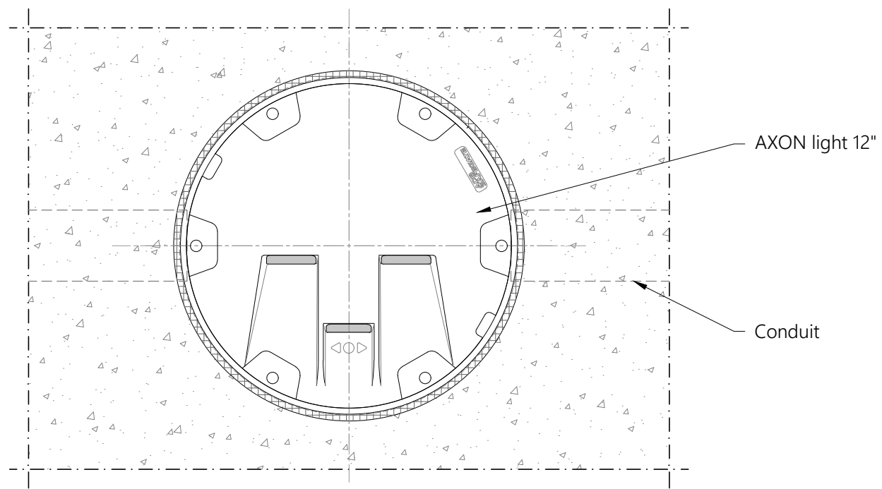
TOP VIEW AXON INSET 12" UNIDIRECTIONAL LIGHT (3 windows) Scale 1/5
