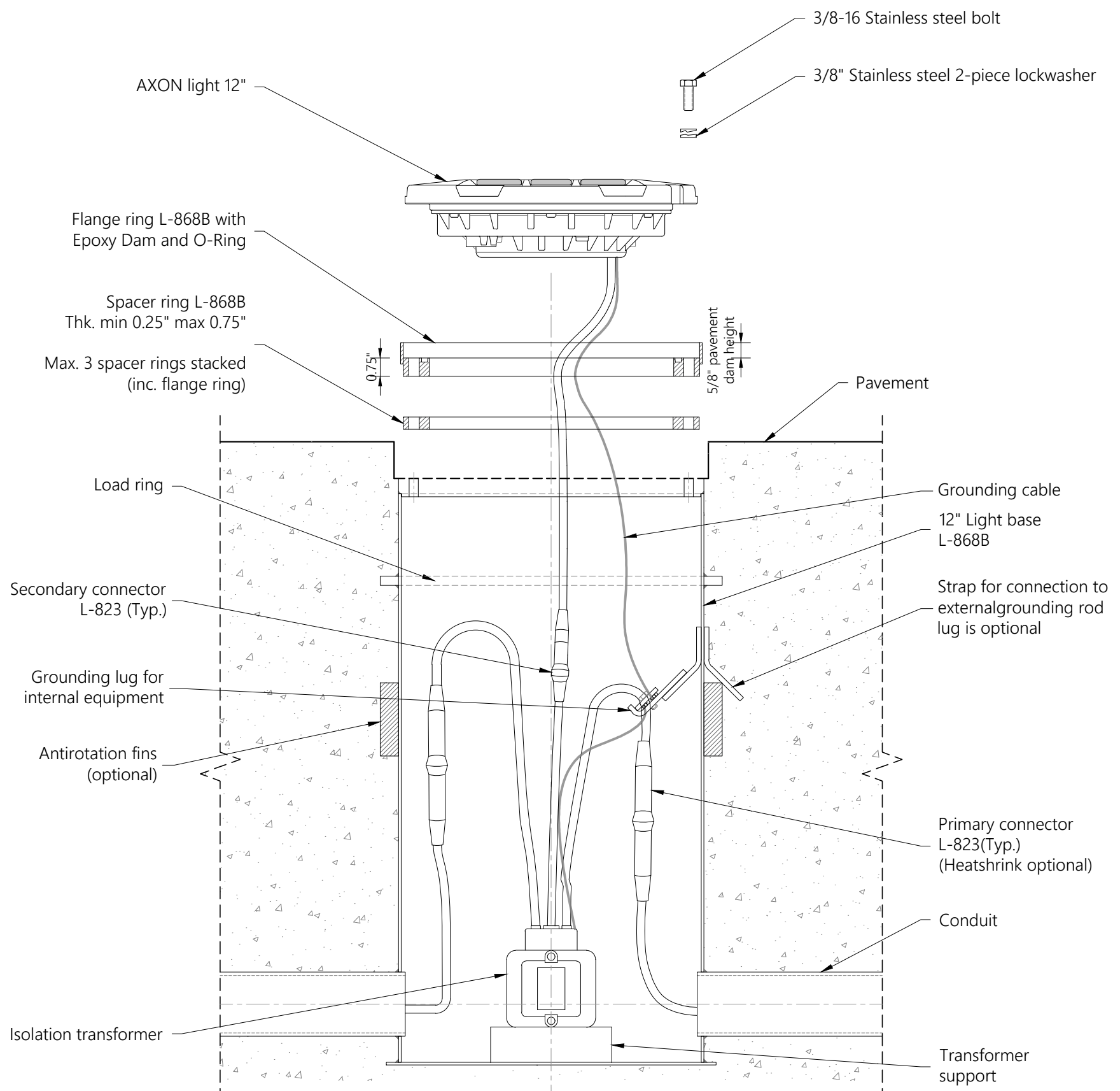
1 PIECE L-868B BASE INSTALLATION AXON INSET 12" UNIDIRECTIONAL LIGHT (3 windows) Scale 1/5
