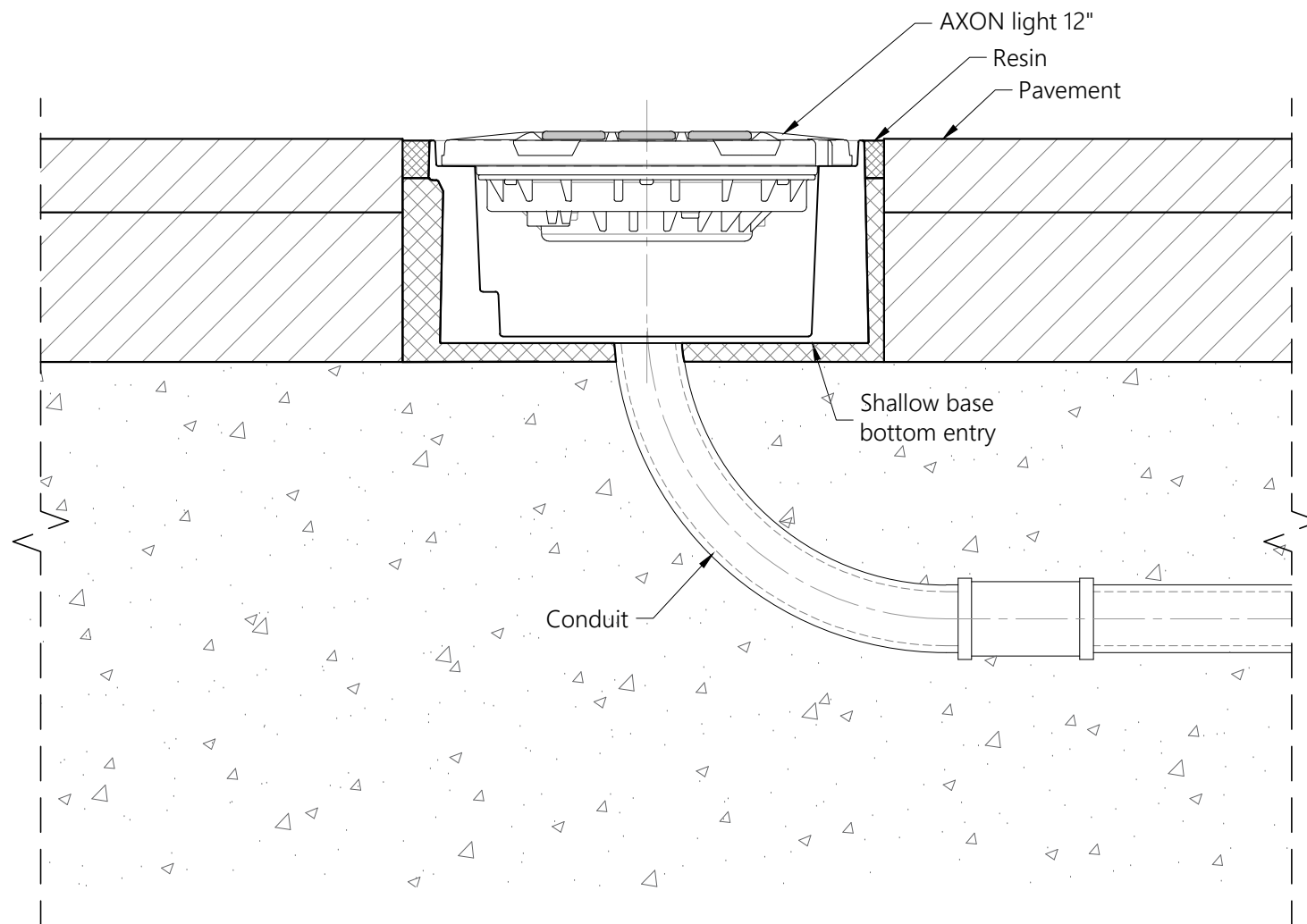
SECTION AXON INSET 12" UNIDIRECTIONAL LIGHT (3 windows) Scale 1/5
