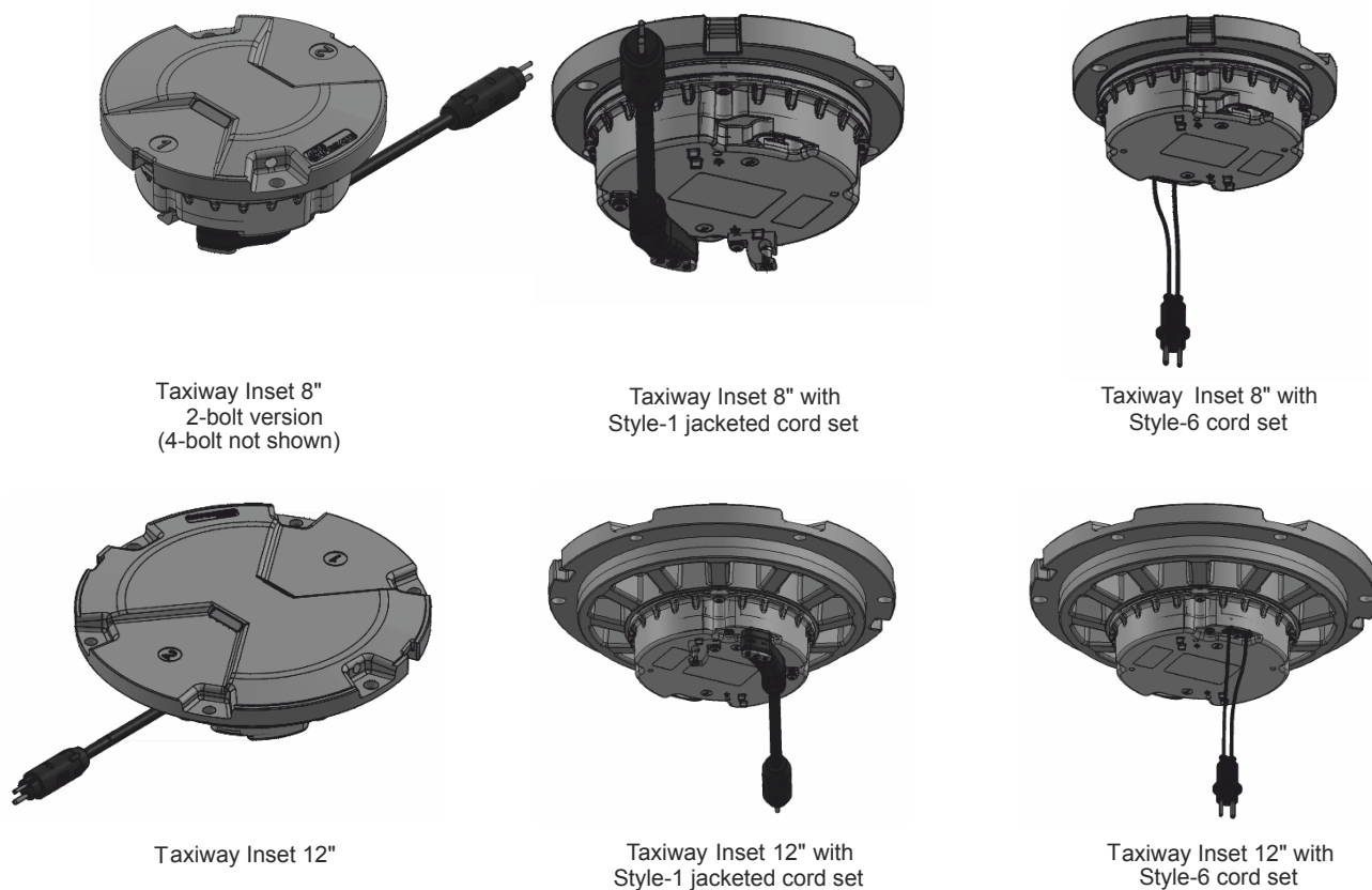
Figure 46: Taxiway Insets, Cord Set Options
