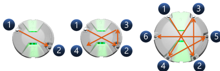
Figure 6: Torque pattern – for 8-inch 2-bolt, 8-inch 4-bolt and 12-inch 6-bolt
