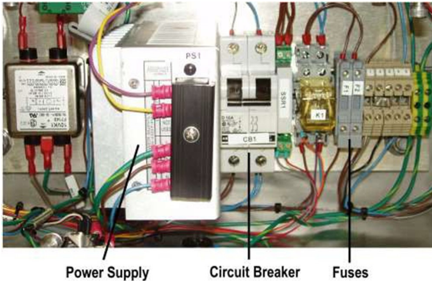
Figure 15. DIN Rail Components
