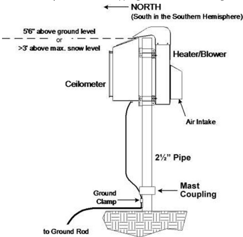
Figure 7. Ceilometer Mounting
