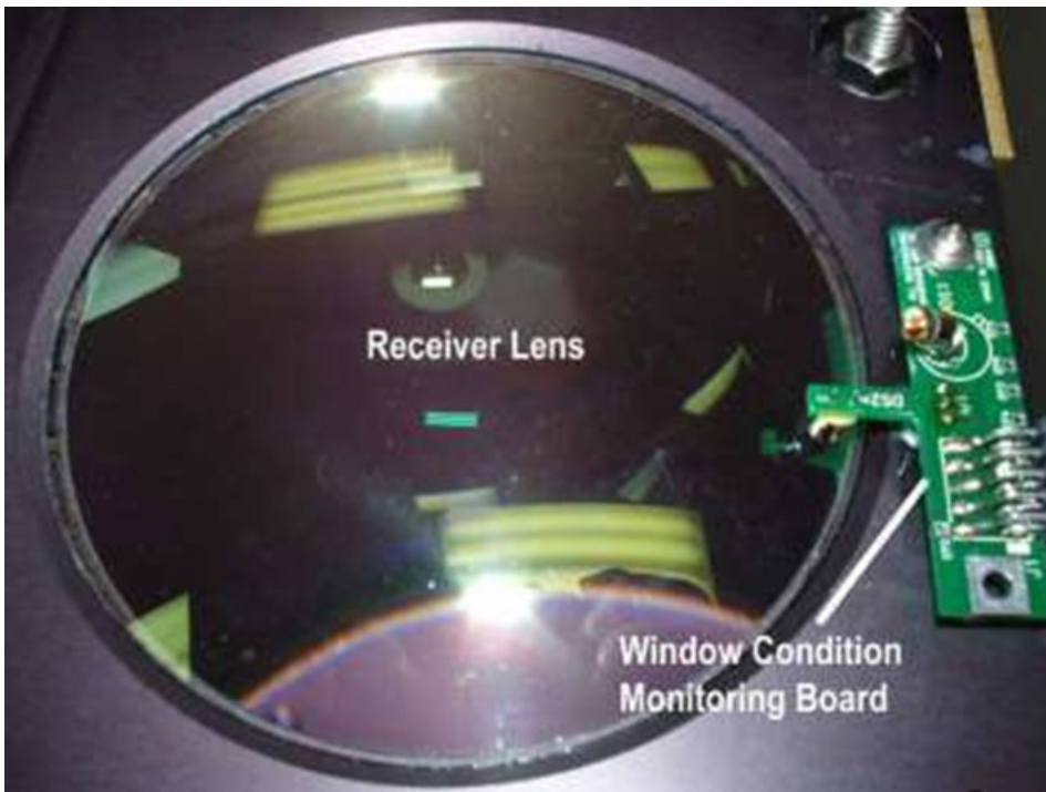
Figure 3. Window Condition Monitoring Board
