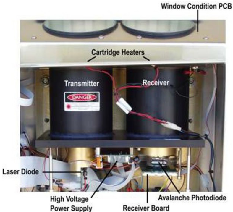
Figure 2. Optical Module
