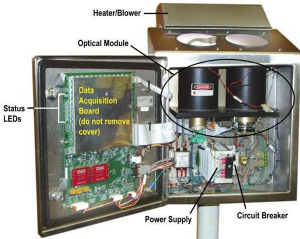
Figure 1. Ceilometer Components
