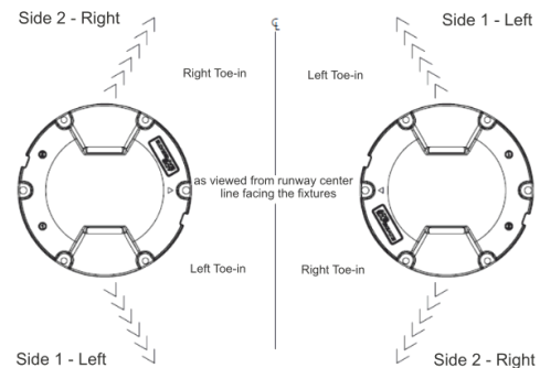
Figure 2. Bidirectional – side 1 and side 2
