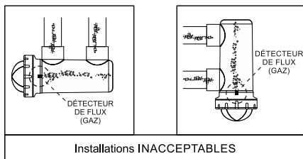
Installations INACCEPTABLES
