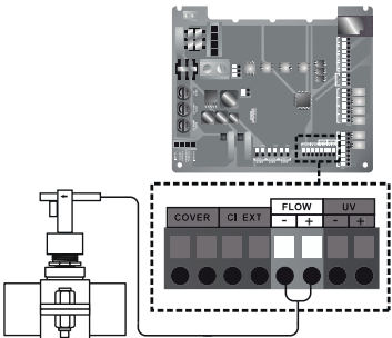
Connecting the paddle sensor (flow switch) to the main board.
