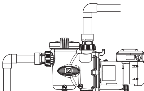
FIGURE 2 - INSTALLATION CORRECTE
