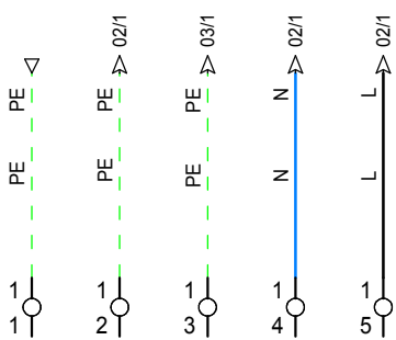
POWER SUPPLY 1PH+N
