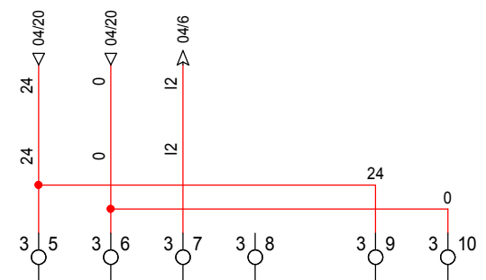
UVC SENSOR 0-10V
