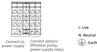
Terminal block for single phase power supply
