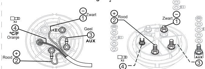
AUX (gassensor)
