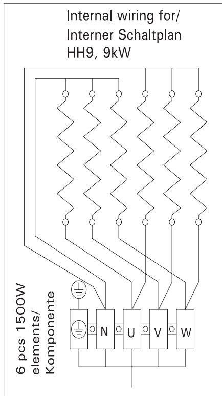
The heater's electrical connections
