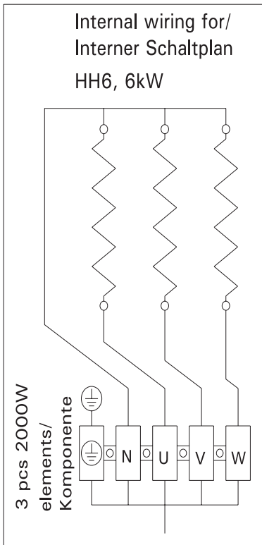
The heater's electrical connections
