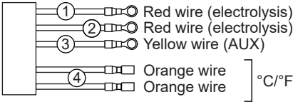
Connecting the gas flow sensor to the device.
